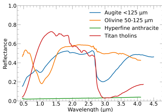
Fig. 1. Individual spectra – between 0.4 and 4.7 \mu\text{m} – of the end members used for this work.
