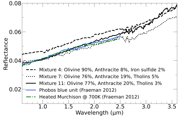
Fig. 7. Spectra of mixtures 4, 7, and 11 compared to the Phobos blue unit CRISM spectrum from Fraeman et al. (2012).
