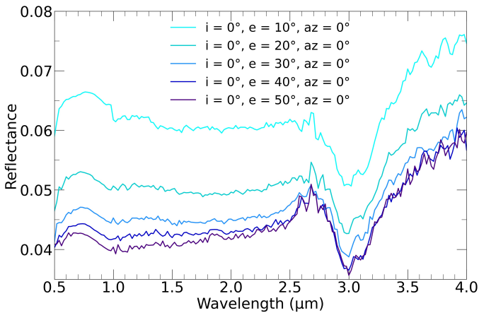
Fig. 11. Effect on phase angle on the reflectance on mixture 16: 68% olivine, 17% anthracite, and 15% tholins.
