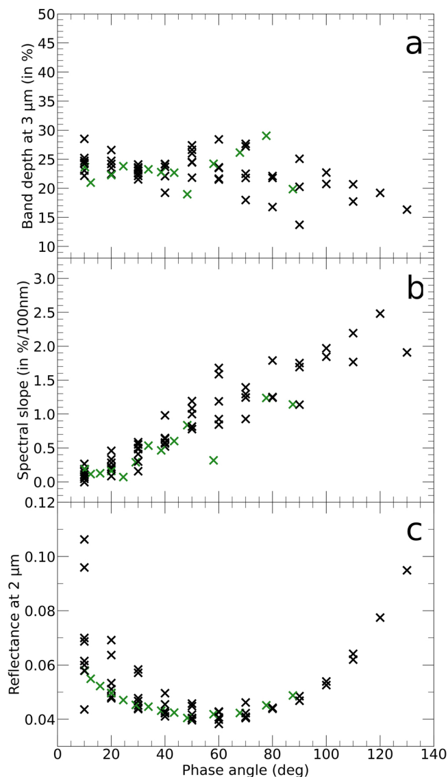
Fig. 12. Geometry observation effects on the 3 \mu\text{m} band depth (a), on the spectral slope evaluated between 1.5 and 2.4 \mu\text{m} (b), and on the reflectance at 2 \mu\text{m} (c) for mixture 16 composed of olivine 68 vol.%, anthracite 17 vol.%, and tholins 15 vol.%. Black crosses represent points for which the azimuth is 0^\circ and green crosses are for an azimuth of 30^\circ .
