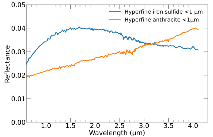
Fig. 2. Spectra of the darkening agents used for this work – anthracite and iron sulfide.
