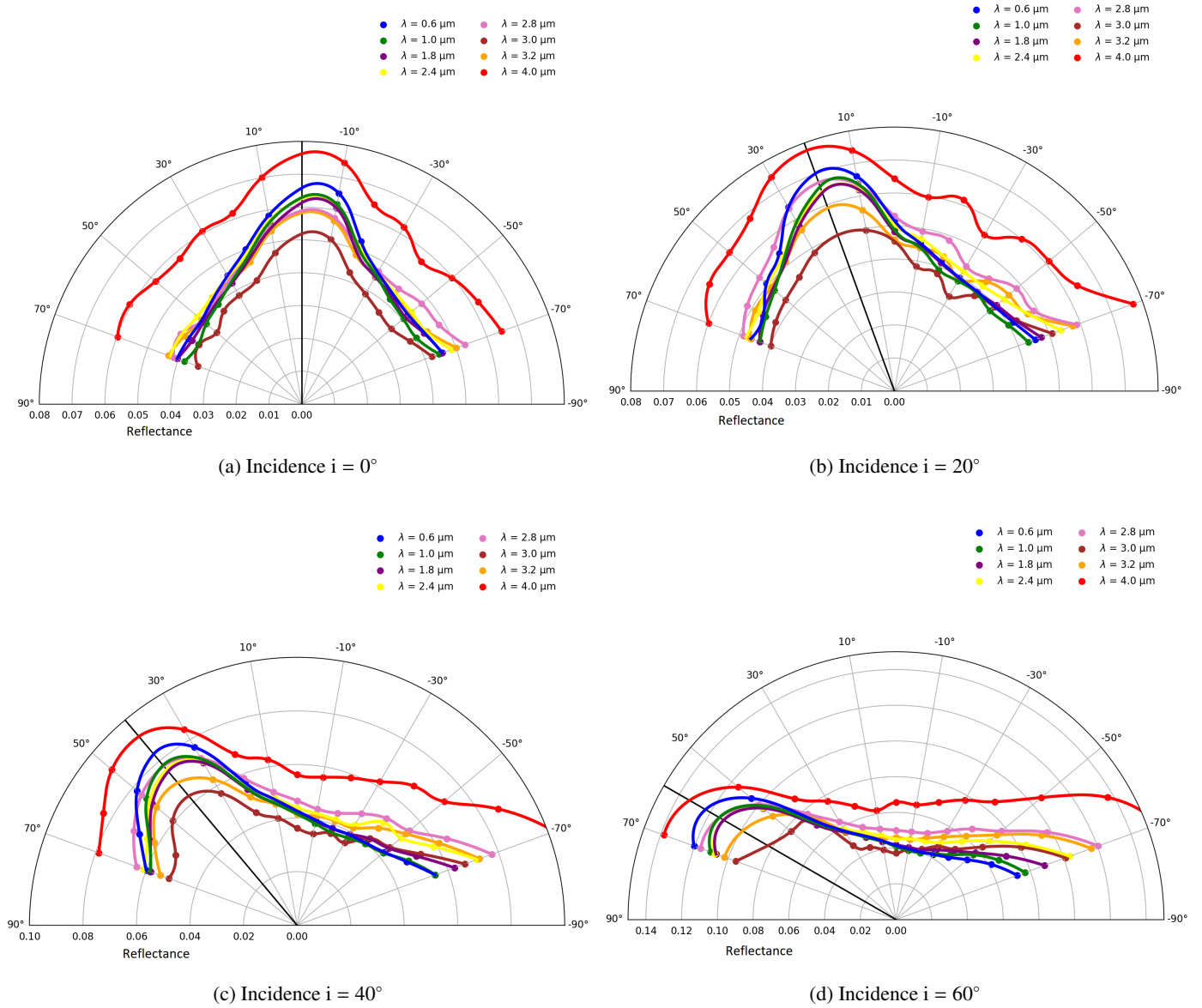
Fig. 10. Reflectance of the mixture 16 in polar coordinates with emergence angle variations from -70^\circ to +70^\circ and at different wavelengths. The straight black line represents the incidence angle.
