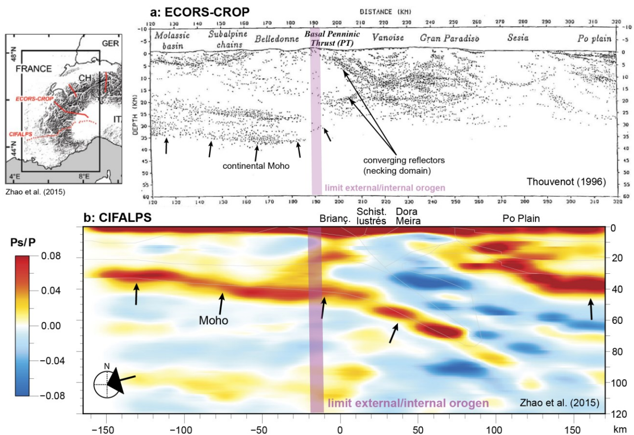
Figure 3. (a) ECORS-CROP seismic profile in depth (modified after [73]). (b) Synthetic common conversion point depth section from the China-Italy-France Alps seismic survey (CIFALPS; modified after [74]). Abbreviation: Brianç.: Briançonnais.
