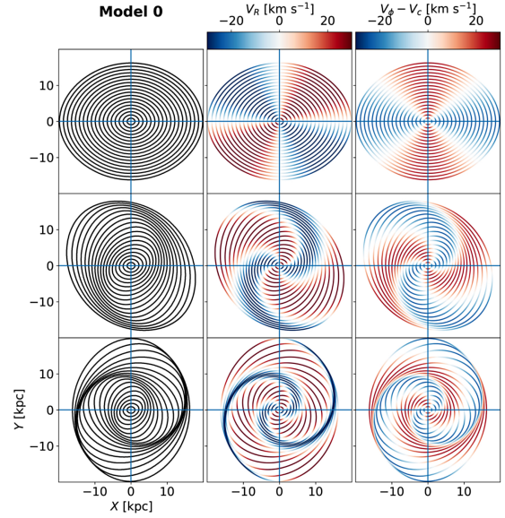
Fig. 2. Rotated ellipses after Kalnajs (1973). Top panel: a series of orbits in the reference frame of \omega - \frac{1}{2}\kappa for which the orbits close. In the first, second and third column, we plot the orbits, the orbits coloured as a function of radial velocity ( V_R ), and as a function of azimuthal velocity ( V_\phi - V_c ), respectively. Two bottom rows: the same but for increasingly rotated ellipses.
