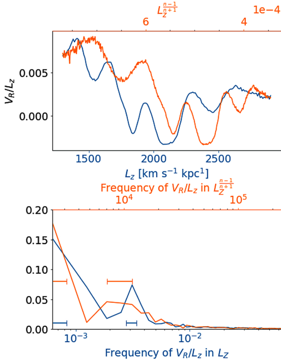
Fig. 26. Frequency analysis of the V_R wave in the MW data. The plot is built as in Fig. 12. The orange curves are for n = 0 , which is one example of the different cases examined. The horizontal error bars indicate the uncertainty in the peaks frequency (see text for details).
