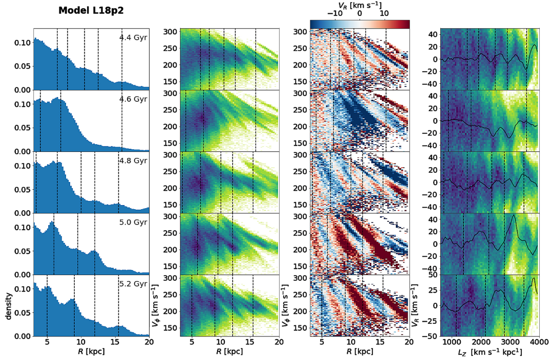
Fig. 19. Ridges and waves for Model L18p2. The structure of the panels is as for Fig. 6.
