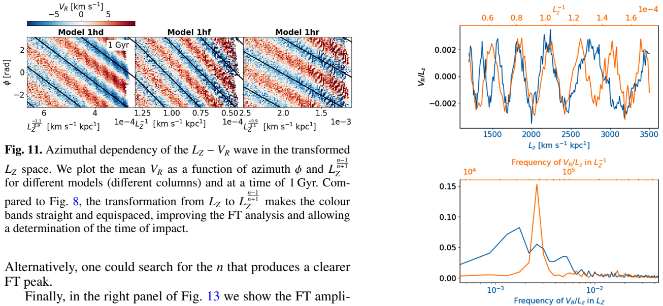
Fig. 12. Example of frequency analysis of the V_R wave for the Model 1hf at time t = 2 Gyr. Top : blue line is the average V_R as a function of L_Z , while the orange line is in the scale of L_Z^{-1} , shown in the top horizontal axis. Bottom : Fourier amplitude as a function of frequency in L_Z (blue and bottom axis) and in L_Z^{-1} (orange, top axis). The frequencies are in units of (\text{km s}^{-1} \text{kpc}^{-1})^{-1} (blue) and \text{km s}^{-1} \text{kpc}^{-1} (orange).
