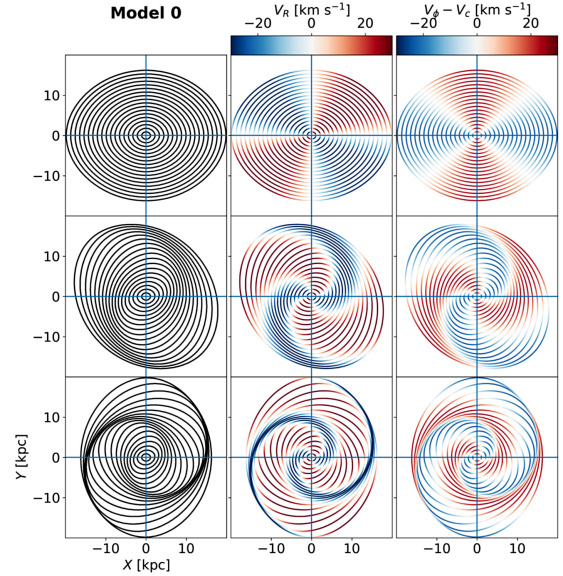
Fig. 2. Rotated ellipses after Kalnajs (1973). Top panel: a series of orbits in the reference frame of \omega - \frac{1}{2}\kappa for which the orbits close. In the first, second and third column, we plot the orbits, the orbits coloured as a function of radial velocity ( V_R ), and as a function of azimuthal velocity ( V_\phi - V_c ), respectively. Two bottom rows: the same but for increasingly rotated ellipses.
