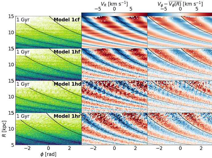
Fig. 4. Spiral arms of different models in polar coordinates. We show the \phi - R projection at 1 Gyr, in density ( left column ), coloured by average radial velocity V_R ( middle ) and average V_\phi - \overline{V_\phi(R)} ( right ). The black lines show the predicted location of the spiral arms.
