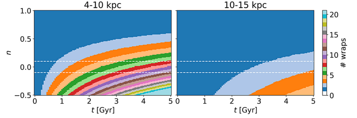
Fig. 5. Number of spiral wraps. We show in colours the expected maximum number of spiral wraps at different radius ranges (4–10 and 10–15 kpc in the first and second columns , respectively) as a function of time t and slope of the circular velocity curve n . We have used 21 for the upper limit of the colour bar but the number of wraps goes beyond this in the bottom part of the left panel .
