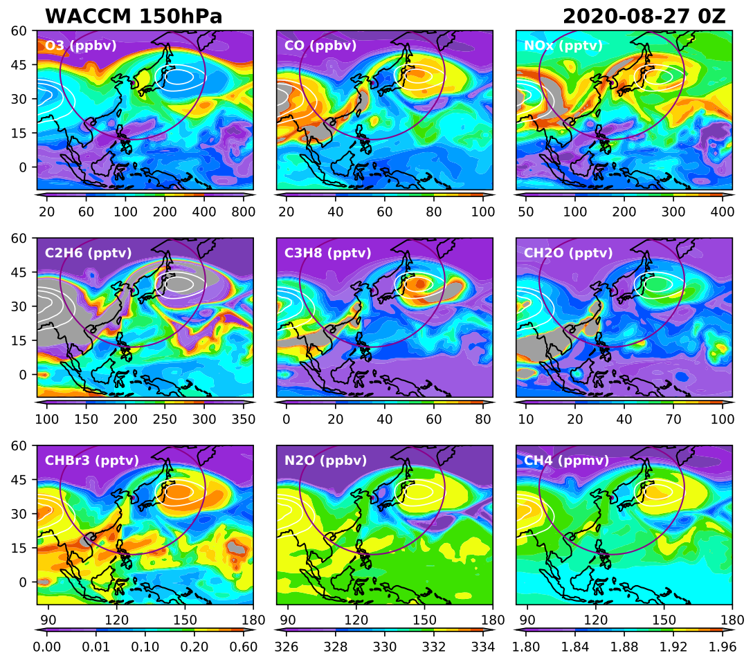
Figure 6. Chemical trace gas content in the shedding air mass from the Whole Atmosphere Community Climate Model (WACCM) at 150 hPa. Example of 27 August 2020. The nine selected species from WACCM highlight the impact of the shedding event on the composition of the UT near the tropopause. Selected geopotential height (GPH) contours (14,300, 14,340, and 14,380 m), at 150 hPa are overlaid to indicate the anticyclone shedding.
