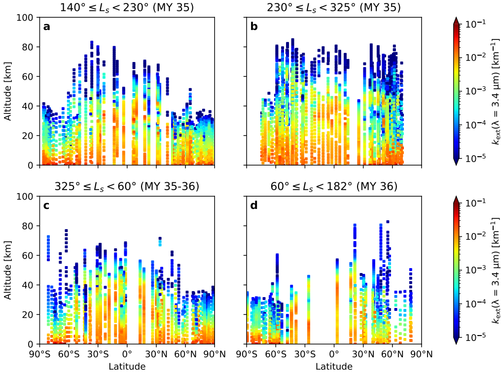
Figure 7. Vertical profiles of the measured opacity of the Martian atmosphere ( k_{\text{ext}} = d\tau/dz , in \text{km}^{-1} ) at 3.4 \mu\text{m} as observed by ACS-MIR between L_s = 140^\circ (MY 35) and L_s = 182^\circ (MY 36) as a function of the latitude of the observation. To highlight the latitudinal variations of the clouds by getting rid of their seasonal dependency (discussed in section 3.2), each panel represents the profiles grouped by ranges of L_s .
