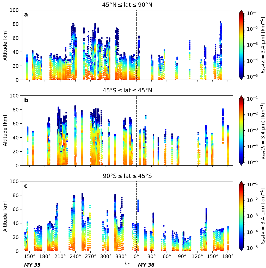
Figure 8. Vertical profiles of the measured opacity of the Martian atmosphere ( k_{\text{ext}} = d\tau/dz , in \text{km}^{-1} ) at 3.4 \mu\text{m} as observed by ACS-MIR over mid-MY 35 to mid-MY 36. To highlight the seasonal variations of the clouds by getting rid of their latitudinal dependency, each panel represents the profiles grouped by ranges of latitude (North/Equatorial/South).
