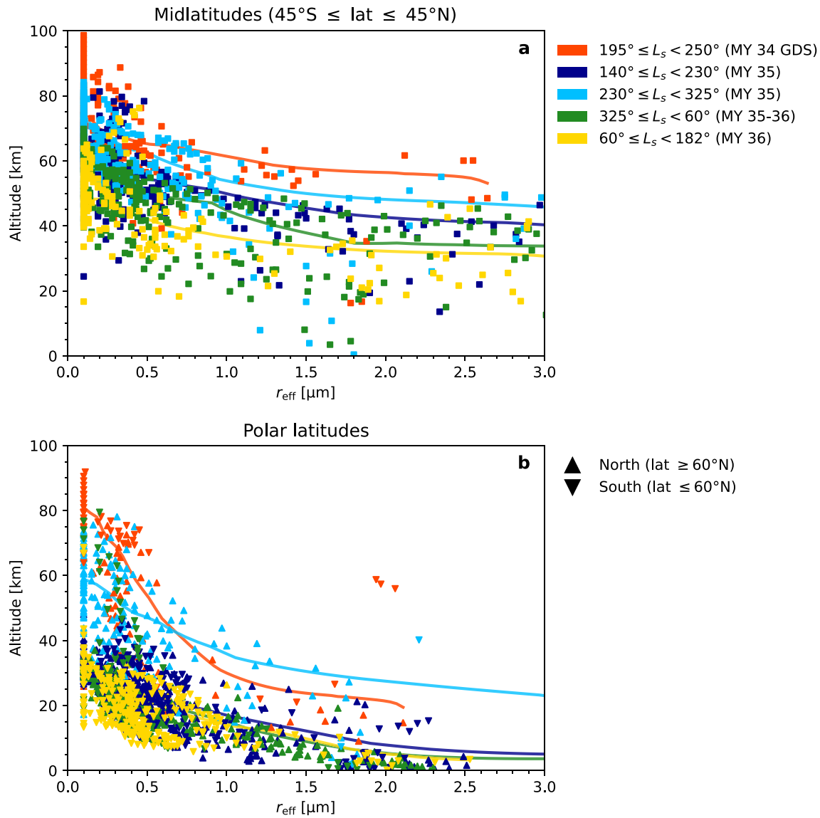
Figure 4. Distribution and size of the water ice crystals within the clouds as a function of their altitude and L_s observation for three ranges of latitude: midlatitudes (panel a) and northern and southern polar latitudes (panel b). The solid lines show the average trend for each range of L_s . Observations acquired during the MY 34 global dust storm (GDS) are shown in red for comparison with data from non-GDS years (MY 35 and 36).
