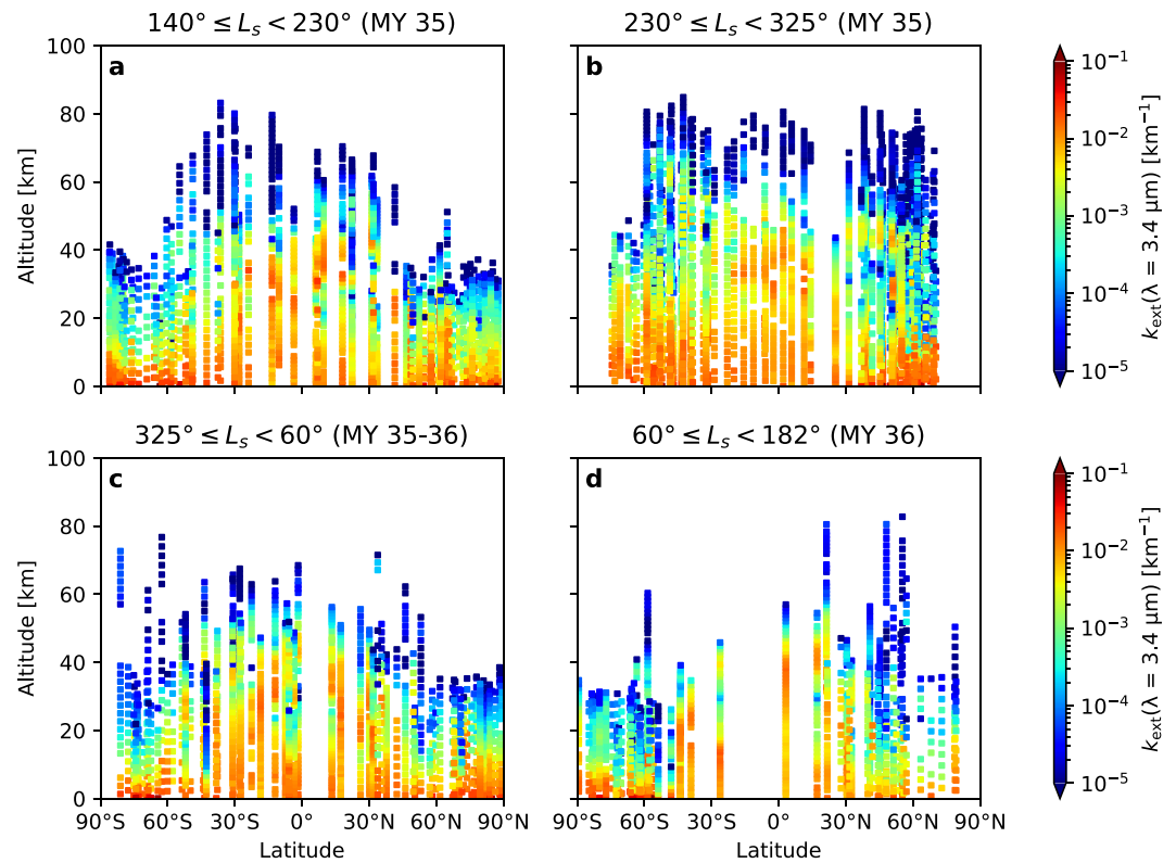
Figure 7. Vertical profiles of the measured extinction of the Martian atmosphere ( k_{\text{ext}} = dz/dz , in \text{km}^{-1} ) at 3.4 \mu\text{m} as observed by ACS-MIR between L_s = 140^\circ (MY 35) and L_s = 182^\circ (MY 36) as a function of the latitude of the observation. To highlight the latitudinal variations of the clouds by getting rid of their seasonal dependency (discussed in Section 3.2), each panel represents the profiles grouped by ranges of L_s .
