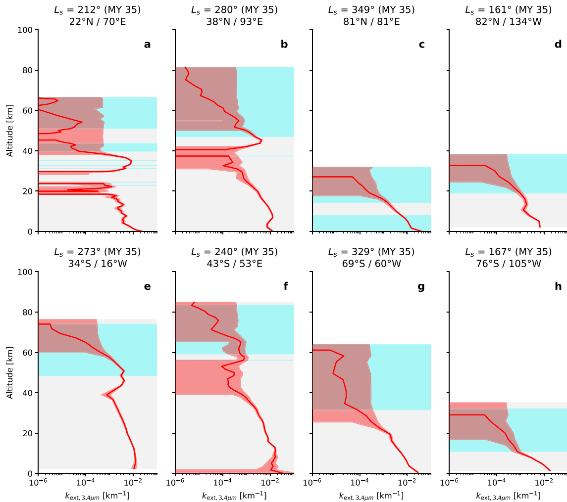
Figure 6. Vertical profiles of the derived extinction coefficient k_{\text{ext}} at \lambda = 3.4 \mu\text{m} from eight different ACS-MIR observations acquired during MY 35 at various latitudes. The light blue areas represent the altitudes where water ice clouds have been identified.
