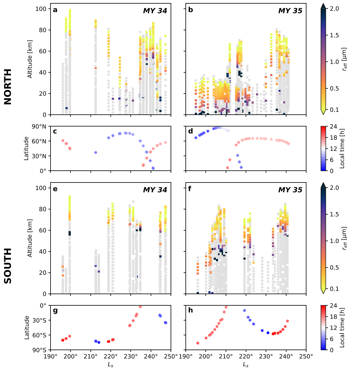
Figure 5. Vertical profiles of water ice clouds in the Martian atmosphere as observed by ACS-MIR between L_s = 190^\circ and L_s = 250^\circ over MY 34 (a and e) and MY 35 (b and f). Panels (c, d, g, and h) indicate the latitudes and local times of the observations presented in panels (a, b, e, and f), respectively. Observations without water ice detection are in gray.
