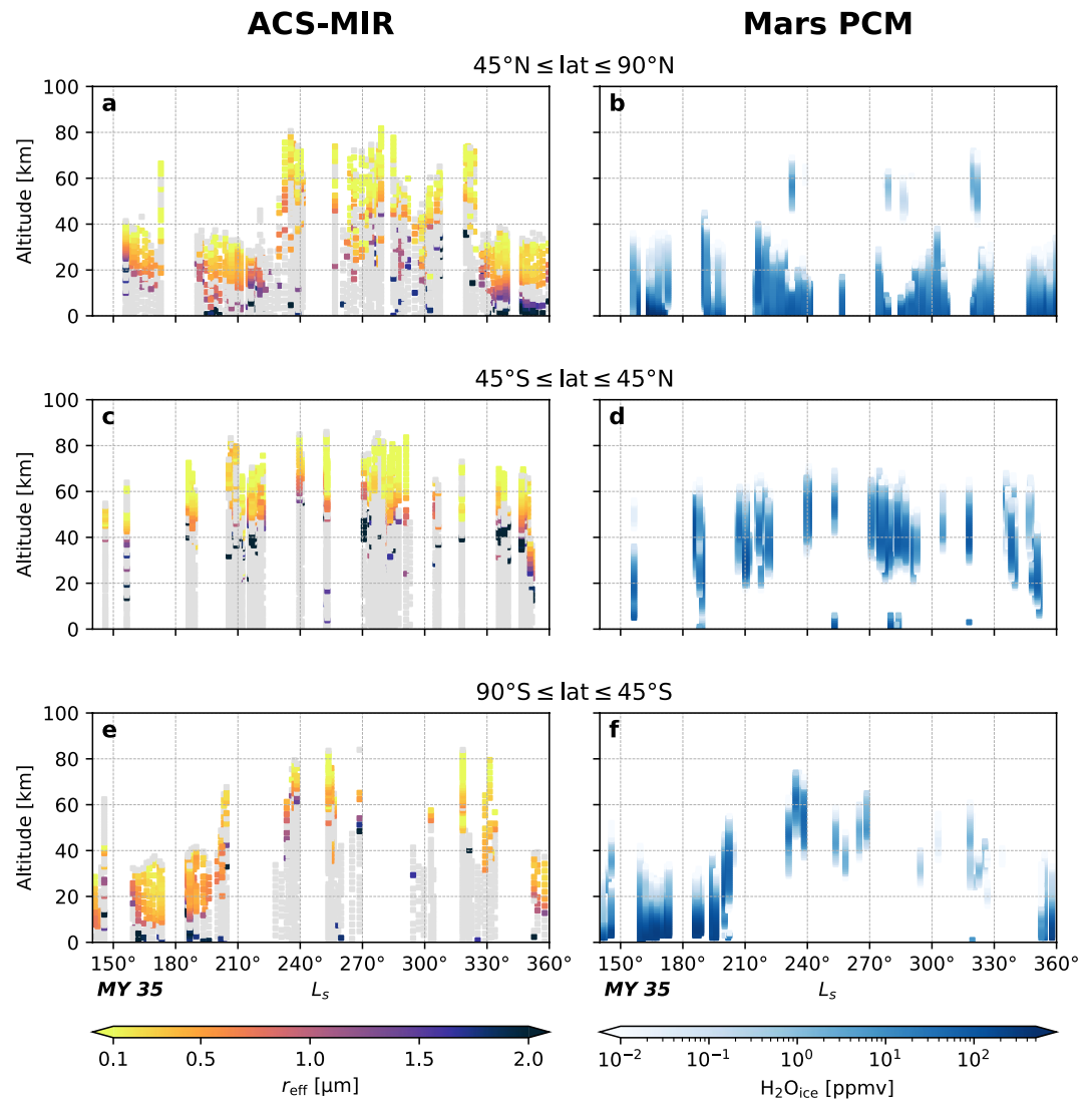
Figure 10. Comparison between the ACS-MIR cloud detections (left) and the water ice clouds predicted by the Mars planetary climate model (right) over the second half of MY 35. Similarly to Figure 8, the profiles are filtered as a function of latitude in each panel to decorrelate between the seasonal and the latitudinal trends.
