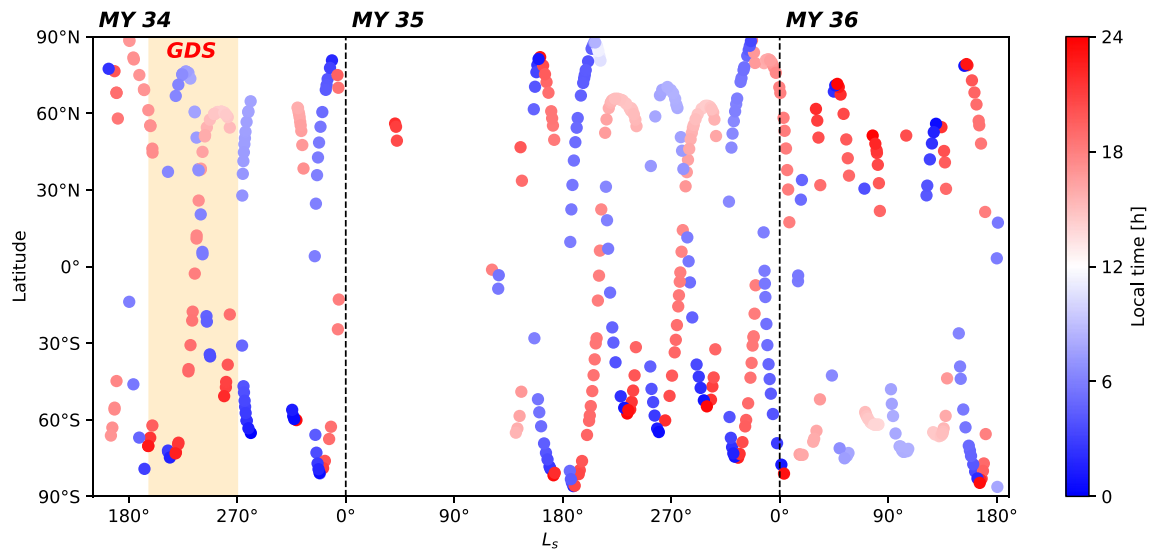
Figure 1. Spatial (latitude) and temporal ( L_s and local time) distribution of the 514 ACS-MIR position 12 observations used in this study. The orange region corresponds to the period of the 2018/MY 34 global dust storm.
