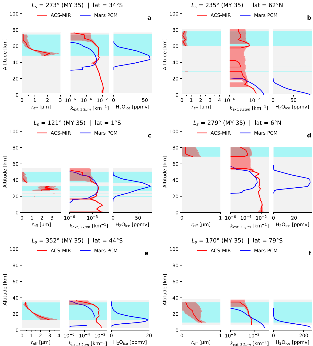
Figure 11. Comparison between the ACS-MIR retrieval (red lines) and the Mars planetary climate model (PCM) prediction (blue lines) for six individual profiles from MY 35. Each panel shows the water ice r_{\text{eff}} retrieved by ACS-MIR (left), the atmospheric extinction ( k_{\text{ext}} ) at \lambda = 3.2 \mu\text{m} (center), and the amount of water ice predicted by the Mars PCM (right). The light blue areas represent the altitudes where water ice clouds have been identified in the ACS-MIR data.
