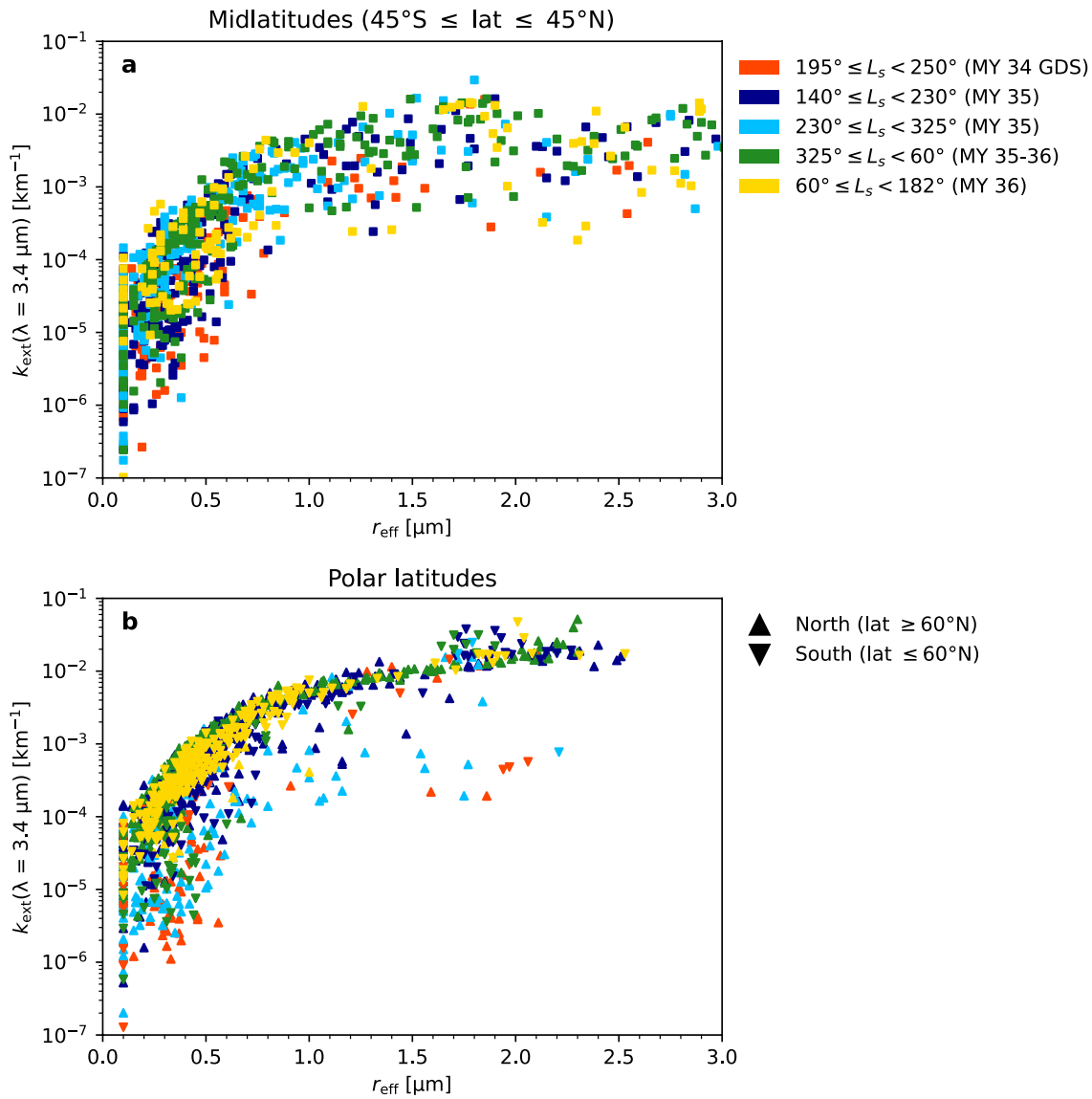
Figure 9. Distribution and size of the water ice crystals within the clouds as a function of their extinction coefficient k_{\text{ext}} and L_s of observation, for three ranges of latitude: midlatitudes (panel a), northern and southern polar latitudes (panel b). Observations acquired during the MY 34 global dust storm are shown in red for comparison with data from non-GDS years (MY 35 and 36).
