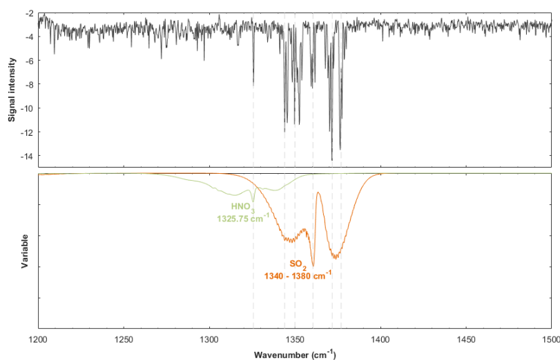
445 446 Figure 14: Top: Example of GMI pseudo spectrum calculated from IASI/Metop-B LIC data during a sulphur plant fire 447 event occurring in Iraq on 24 October 2016 in the evening (PM orbit). Bottom: HITRAN spectroscopic parameter associated 448 with the absorption of different species are shown in colours.
