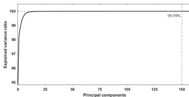
142 Figure 2: Evolution of the explained variance ratio in function of the rank of principal components. 99.99% of the 143 atmospheric variability is depicted by the 150 first eigenvectors.
