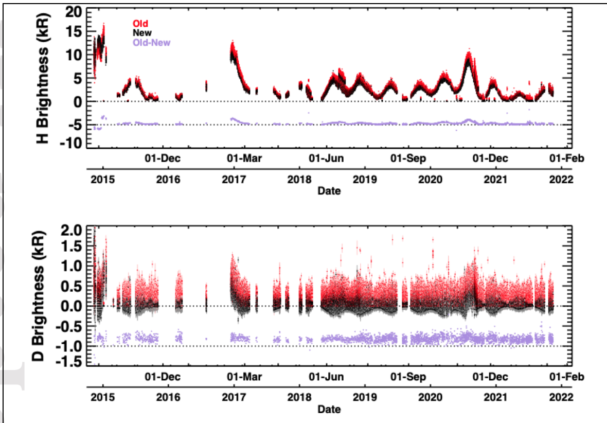
Figure 7. Integrated brightness values for H (top) and D (bottom) Lyman- \alpha emissions for all frames from observations spanning orbits 240 – 15794 (Nov 12, 2014 – Feb 14, 2022) when the IUVS line of sight is pointed at the disk. The old pipeline brightness values are plotted in red; the new values are in black. The differences between the old and new brightness values are shown in purple, offset by -5 and -1 kR for H and D, respectively, for visibility. The 1\text{-}\sigma uncertainties in the integrated brightness values are shown as thin vertical lines extending from each data point. The horizontal dotted lines indicate the zero-value brightness levels. Scientific analysis of this data would benefit from co-addition to maximize the signal-to-noise ratio.
