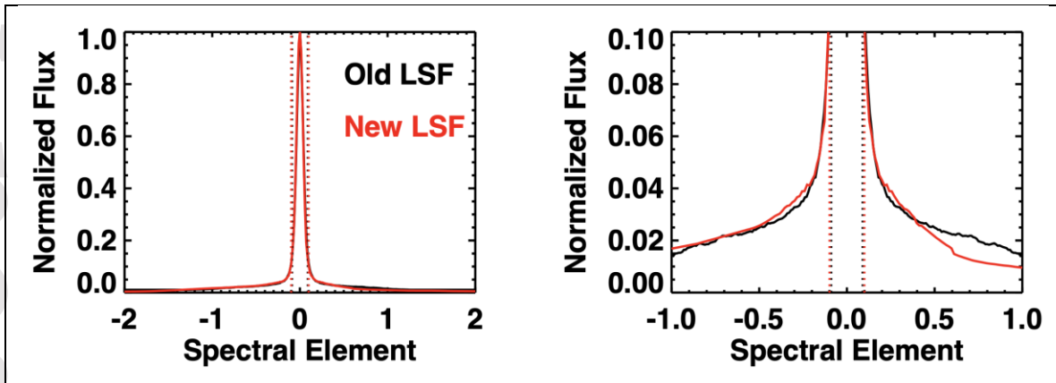
Figure 3. (Left) A comparison of the IUVS/Echelle normalized line spread functions. The old LSF (black) is derived from laboratory-generated spectra. The new LSF (red) is derived from in-orbit disk-pointed spectra. (Right) The zoomed-in view of the two LSFs are compared to highlight differences in the spectral wings. The dotted vertical lines denote the regions of full-width at half-max for each LSF and overlap for both functions. The functions are normalized to peak values and the x-axis units are in binning-specific spectral element, d\lambda , described in the text.
