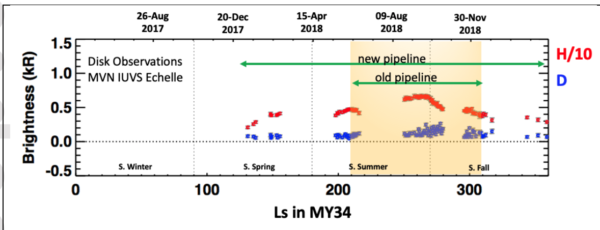
Figure 10. The new on-disk derived Lyman- \alpha brightness values versus solar longitude (Ls) for D (blue) and H (red, divided by 10 to facilitate comparison) emissions obtained with MAVEN/IUVS/Echelle in Mars Year 34 (May 5 th , 2017 – Mar 23 rd , 2019). The yellow shaded region indicates the seasonal range where D emission brightness values were considered reliable, as derived with the old pipeline. The upgraded pipeline produces a broader range (all plotted values) of reliable D detections and facilitates improved science interpretations.
