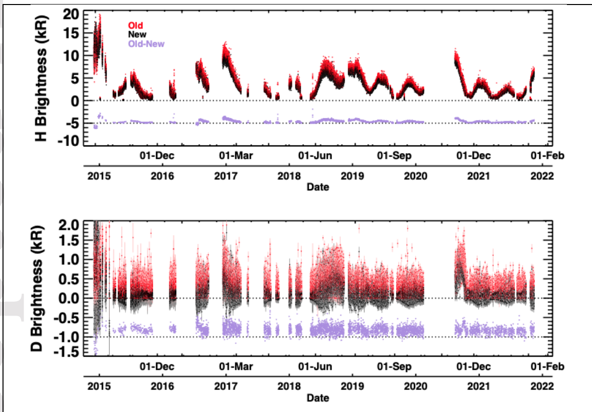
Figure 8. Integrated brightness values for H (top) and D (bottom) Lyman- \alpha emissions from all frames of observations spanning orbits 240 – 15794 (Nov 12, 2014 – Feb 14, 2022) when the IUVS line of sight is pointed at the limb, for observations where the minimum ray height at the tangent point is between the planetary disk and 300 km altitude. The old pipeline brightness values are plotted in red; the new values are in black. The differences between the old and new brightness values are shown in purple, offset by -5 and -1 kR for H and D, respectively, for visibility. The 1-\sigma uncertainties in the
