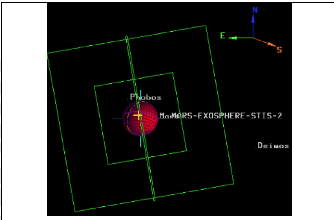
Figure 1. The observational configuration for Mars (red shaded disk) obtained from the HST Phase II target confirmation chart for the calibration data used in this work. The large green box denotes the full 50'' \times 50'' field of view of the CCD detector for a broad wavelength range. The inner green box denotes the 25'' \times 25'' field of view of the HST/STIS MAMA detector used in this work. The narrow green rectangle denotes the 52'' \times 0.5'' HST/STIS aperture. The pale blue cross is the center of the HST/STIS FOV and is centered on the disk of Mars. The purple arc denotes the planetary equator, and the orange arc represents the terminator line. The axes on the top right indicate the location of the Sun (S), terrestrial North (N) and terrestrial East (E). Labels for the Martian moons are indicated next to the orange dots of their location in the observation. The labels for Mars and Mars-Exosphere-STIS-2 (assigned by the observer during Phase II planning) are indicated. The orange cross indicates the location of the MAVEN/IUVS/ECH line of sight for the simultaneous observations utilized for cross-calibration.
