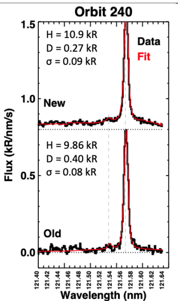
Figure 5: Comparison of new (top) and old (bottom) MAVEN echelle data reduction pipeline fitting algorithms for on-disk observation of the first frame of orbit 240 (Nov 12, 2014). Data that has been reduced is shown in black and fits to the data are shown in red. The emission line centers of D Lyman- \alpha and H Lyman- \alpha are indicated by the vertical dashed grey lines at 121.535 and 121.567 nm, respectively. A horizontal dotted line indicates the zero-level emission for each spectrum. The top spectrum is offset in vertical coordinates for clarity of comparison and both spectra use the same x-axis range (wavelength in nm). The brightness of each emission, integrated over the aperture, uses the HST calibration and is shown on the left legend. The uncertainty ( \sigma ) is derived from a region on the reduced spectrum that is far from the H and D Lyman- \alpha emissions.
