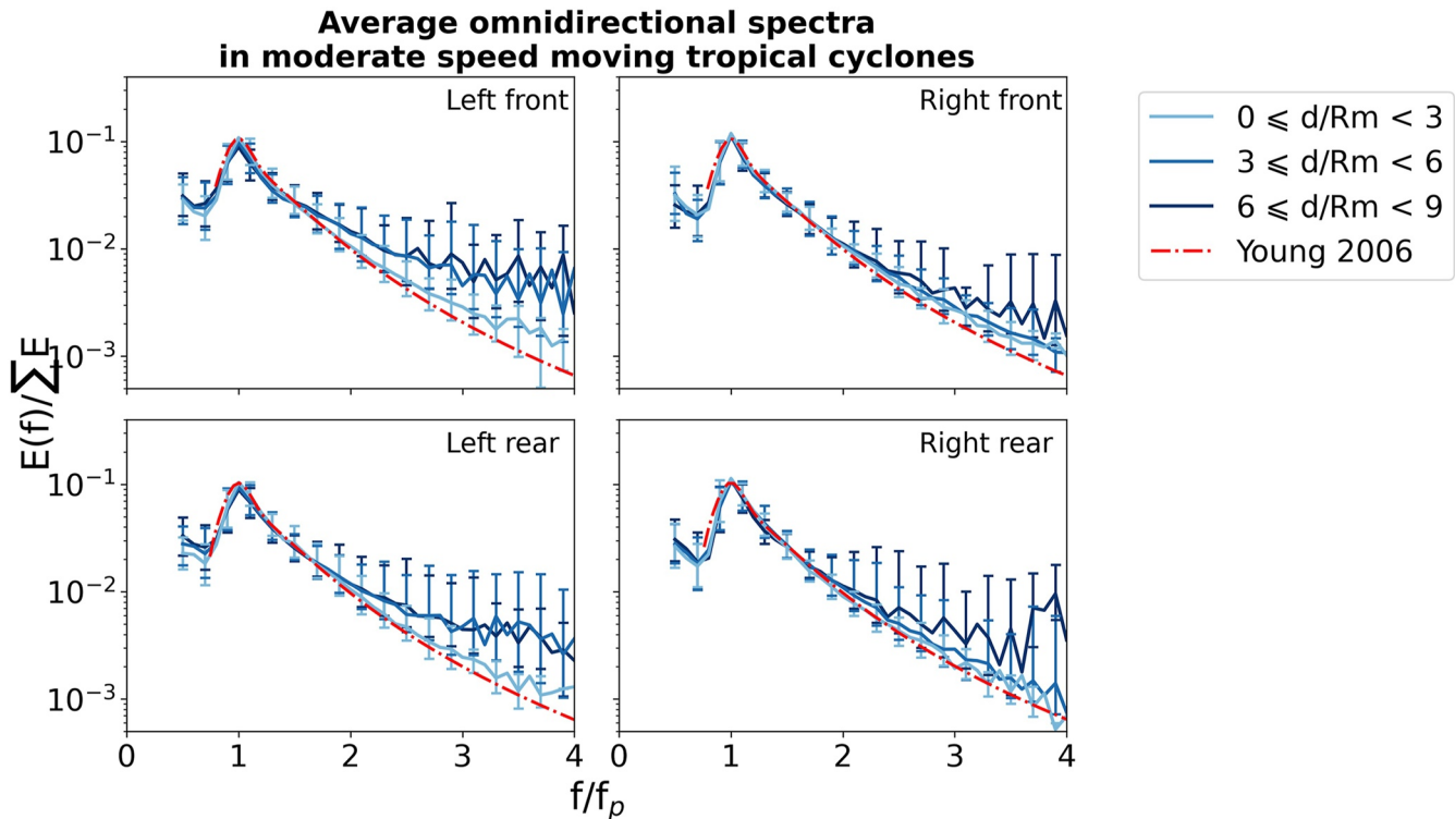
Figure 11. Average omni-directional spectra as a function of the normalized frequency ( f/f_p ) for each quadrant under moderate speed tropical cyclone conditions. The energy of the spectra is normalized with the total energy. The color of the lines, squares and error bars correspond to the distance ranges as reported in the legend. The red dashed-dotted line corresponds to the JONSWAP spectrum adjusted by Young (2006).
