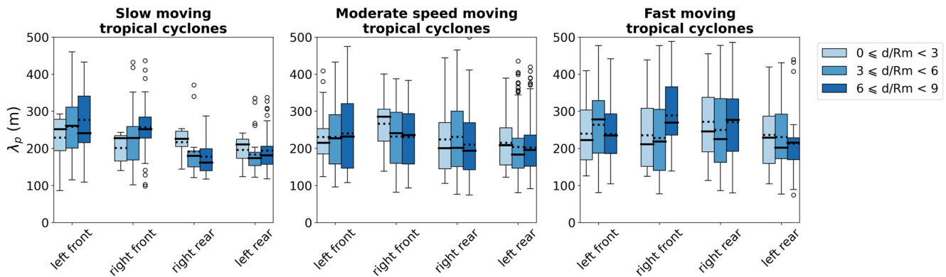
Figure 4. Boxplots showing the distribution of the dominant wavelength ( \lambda_p ) of the whole spectrum for slow (left panel), moderate speed (middle panel) and fast (right panel) moving tropical cyclones in every quadrants as reported on the horizontal axis. The figure characteristics are the same as in Figure 3.
