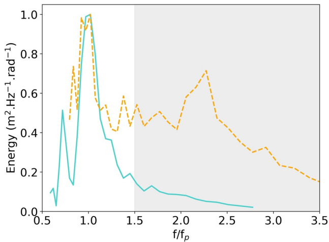
Figure 12. Examples of Surface Wave Investigation and Monitoring (SWIM) omni-directional frequency wave height spectrum as a function of f/f_p obtained in moderate speed moving tropical cyclone at distances larger than 6 R_{max} . The gray area indicates the portion of the spectrum over which is calculated the n factor. The spectra are normalized according to their respective maximum of energy.
