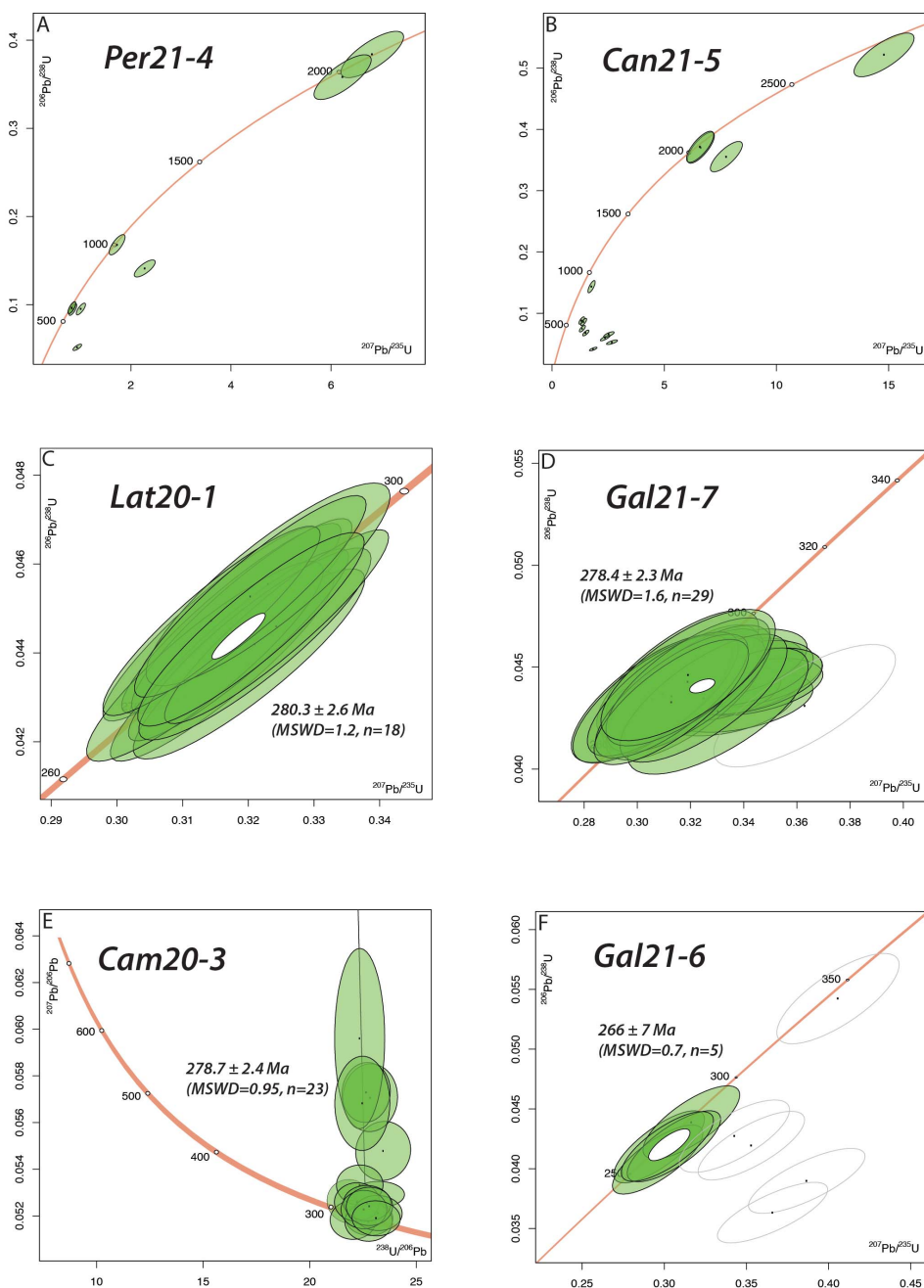
Figure 8. (A) Wetherill concordia diagram for sample Per21-4; (B) Wetherill concordia diagram for sample Can21-5; (C) Wetherill concordia diagram for sample Lat20-1; (D) Wetherill concordia diagram for sample Gal21-7; (E) Tera-Wasserburg concordia diagram for sample Cam20-3; (F) Wetherill concordia diagram for sample Gal21-6. MSWD = Mean Square Weighted Deviation. n = number of analyses used to calculate the U–Pb dates. All MSWD are calculated for concordance + equivalence. Grey ellipses were not used for age calculation.
