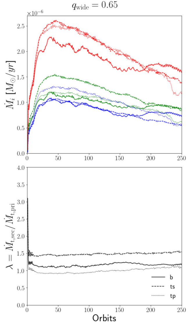
Figure A3. Accretion rates and \lambda = (\dot{M}_{t,\text{sec1}} + \dot{M}_{t,\text{sec2}})/\dot{M}_{t,\text{pri}} factors measured in the triple simulations run to test longer integration times. In the upper panel are plotted the total accretion rate of the system (red) and the accretion rate of the secondary (green) and primary (blue) star. In the lower panel is plotted the ratio between the accretion rates (secondary over primary). The solid, dashed, and dotted lines refer to the binary ( b65 ), ts triple ( ts65 ), and tp triple ( tp65 ) simulations, respectively. The secondary (primary) accretion rate for the ts ( tp ) triple system is the sum of the accretion rates of the small binary stars.
