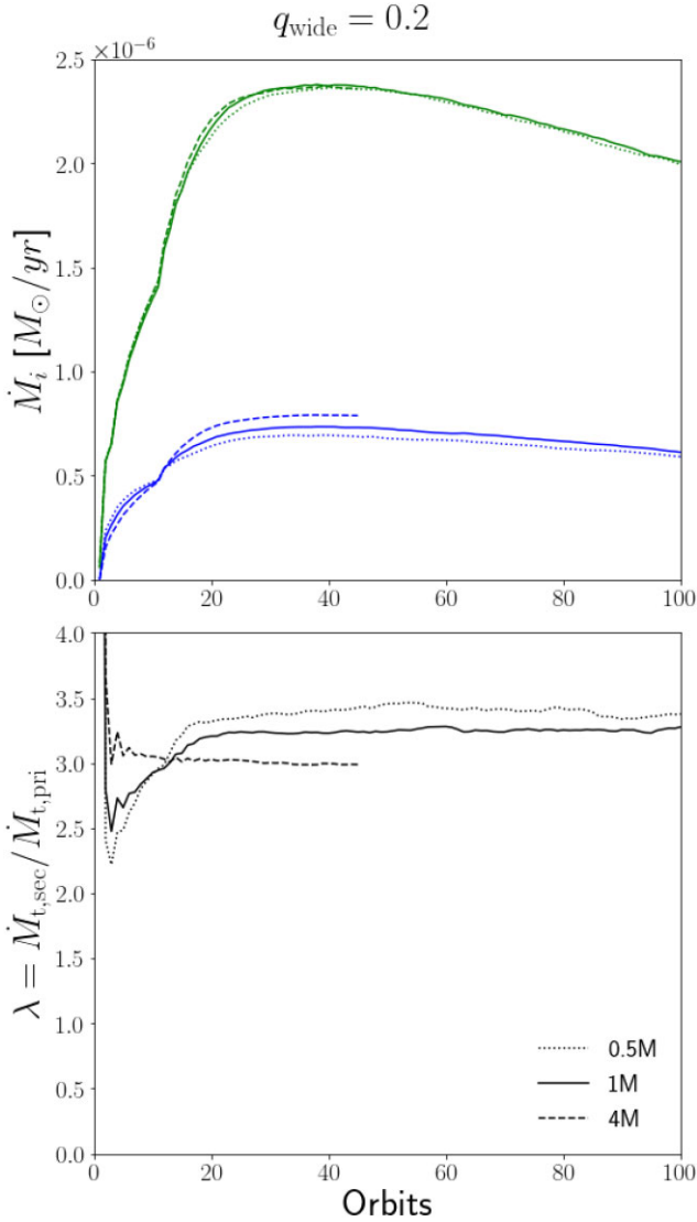
Figure A2. Accretion rates and \lambda = (\dot{M}_{t,\text{sec1}} + \dot{M}_{t,\text{sec2}})/\dot{M}_{t,\text{pri}} factors measured in the triple simulations run to test the resolution. In the upper panel are plotted the accretion rates of the secondary (green) and primary (blue) star. In the lower panel is plotted the ratio between the accretion rates. The solid line refers to the reference simulation ts2 . Dotted and dashed lines refer to the lower and higher resolution simulations, respectively. The secondary accretion rate for the triple system is the sum of the accretion rates of the small binary stars.
