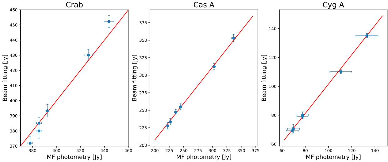
Figure 6. Comparison between the beam-fitting photometry used for the Wide Survey map calibration (Rubino-Martín et al. 2022) and the MF photometry used in this paper for the six MFI detectors (corresponding to horns 2, 3, and 4) and for the three calibration sources Crab, Cassiopeia A, and Cygnus A. The red line shows the best linear y = ax fit.
