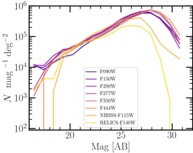
Figure 2. Magnitude number counts from the SE++ extraction in the seven NIRCcam and NIRISS filters. Also overplotted are the HST WFC3/IR F140W number counts from RELICS (Coe et al. 2019; Salmon et al. 2020). The plot illustrates the improvement in depth and the increase of the number of faint sources detected with JWST.
