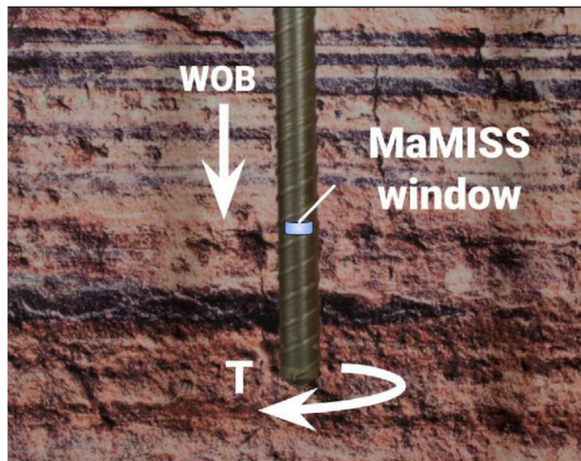
Fig. 3. Cross-section view of drilling into a sedimentary rock. The position of the Ma_MISS window is ~ 22 cm above the drill tip. The weight on bit (WOB) and torque (T) are among the most interesting parameters collected in the drill telemetry, providing information on the mechanical properties of rock layers. Modified from https://bit.ly/3bxe0M9 and Frigeri et al., (2021).
