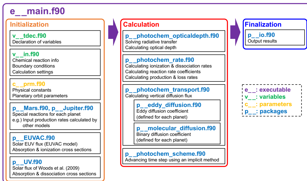
Figure 2 Schematic illustration of the structure of Fortran codes.
