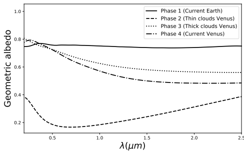
Fig. 4. The planets' geometric albedo's A_G as functions of the wavelength \lambda for the four evolutionary phases.
