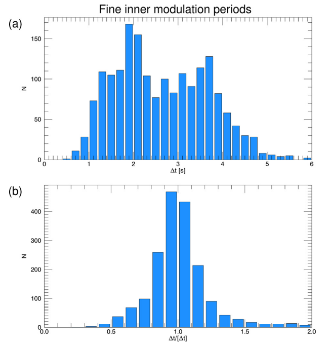
Fig. 6. (a) Histogram of observed fine inner modulation periods of quasiperiodic events. (b) Histogram of observed fine inner modulation periods normalized by median fine inner modulation periods of individual events.
