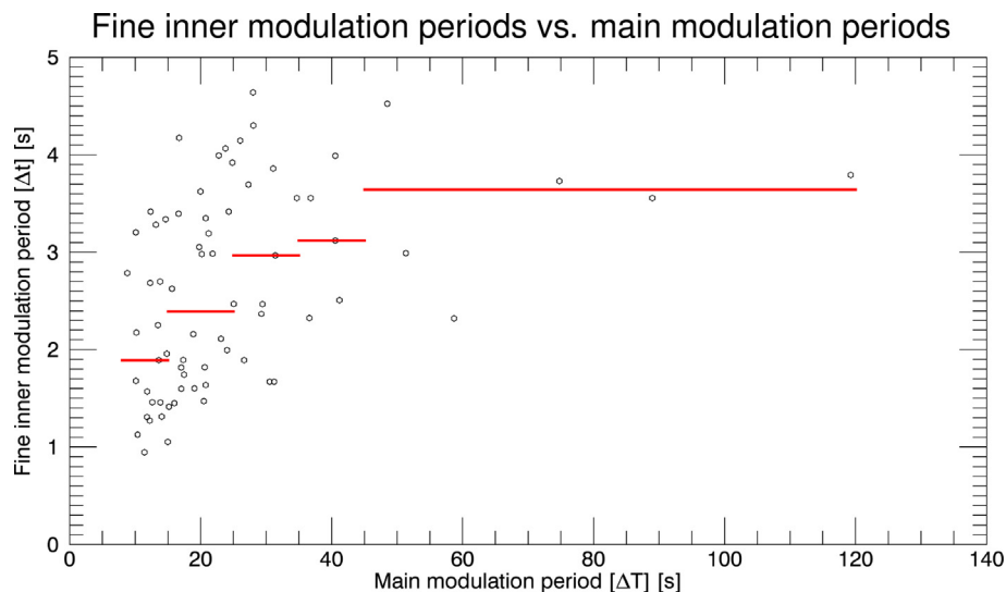
Fig. 8. Median fine inner modulation periods of quasiperiodic events as a function of their main event modulation periods. The horizontal red lines mark the median values in the respective intervals.
