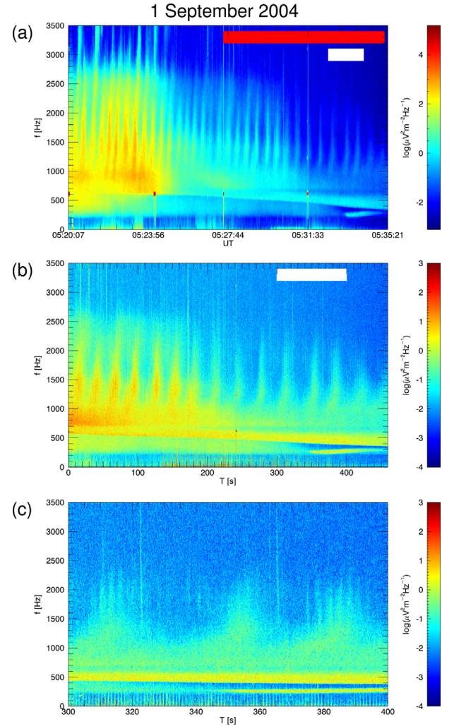
Fig. 1. Example of a quasiperiodic event with a fine inner structure observed on 1 September 2004. (a) Frequency-time spectrogram of power spectral density of electric field fluctuations based on the Survey mode data. (b) Zoomed frequency-time spectrogram of power spectral density of electric field fluctuations based on the Burst mode data corresponding to the time interval marked by the red horizontal bar in panel a). (c) Extra zoomed frequency-time spectrogram of power spectral density of electric field fluctuations based on the Burst mode data corresponding to the time interval marked by the white horizontal bars in panels a), b).
