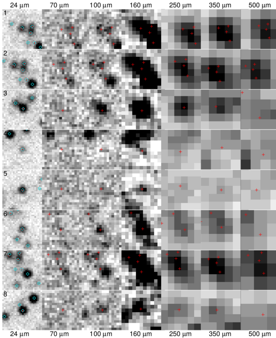
Figure A1. Postage-stamp grey-scale plots showing 30\text{ arcsec} \times 30\text{ arcsec} Spitzer MIPS (24 \mu\text{m} ), Herschel PACS (70, 100 and 160 \mu\text{m} ) and Herschel SPIRE (250, 350 and 500 \mu\text{m} ) images centred on each of the 16 ALMA sources. The ALMA positions are marked by the red crosses, while the blue diamonds mark 24 \mu\text{m} catalogue positions.
