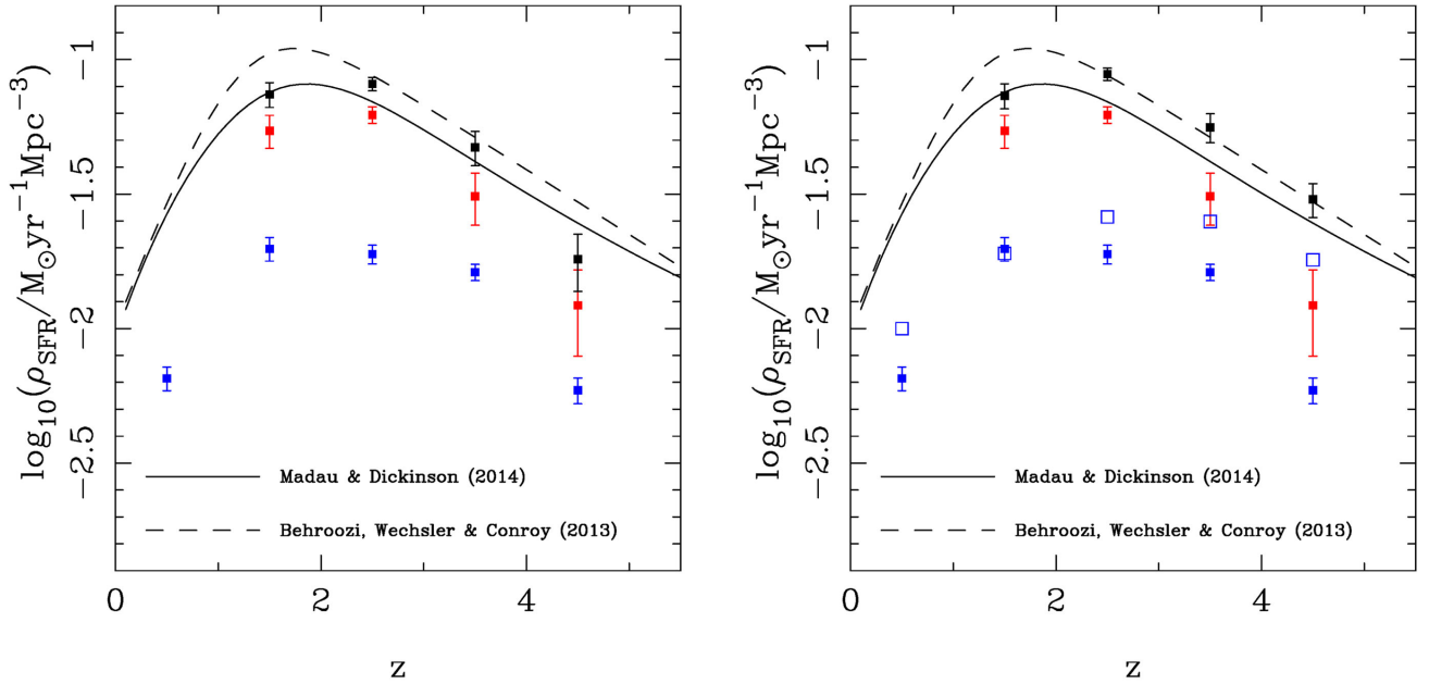
Figure 14. The cosmic evolution of comoving SFR density, \rho_{\text{SFR}} . In the left-hand panel, we plot our new ALMA-derived estimates of \rho_{\text{SFR}}(\text{obscured}) (red points), estimated values of \rho_{\text{SFR}}(\text{visible}) produced by summing the raw UV-derived SFR of the galaxies in the HUDF (blue points) and the values of \rho_{\text{SFR}}(\text{total}) that result from adding these two contributions at each redshift (black points). The solid and dashed curves show two recent parametric descriptions of the evolution of \rho_{\text{SFR}} as derived from the literature by Madau & Dickinson (2014) and Behroozi, Wechsler & Conroy (2013), respectively (scaled to the IMF of Chabrier 2003). In the right-hand panel, we show the impact of including a more complete census of \rho_{\text{SFR}}(\text{visible}) , based on the luminosity-weighted integral of the evolving UV galaxy luminosity function, down to M_{\text{UV}} = -15 (Parsa et al. 2016; Bouwens et al. 2015). In this panel, the values of \rho_{\text{SFR}}(\text{obscured}) are unchanged, but the black points indicating \rho_{\text{SFR}}(\text{total}) now include the more complete (and, at high redshift, higher) census of \rho_{\text{SFR}}(\text{visible}) , as shown by the open blue squares. At z \simeq 2 the agreement with the parametric fit provided by Behroozi et al. (2013) is excellent, and our results indicate that there is a transition from \rho_{\text{SFR}}(\text{visible})/\rho_{\text{SFR}}(\text{obscured}) > 1 , to \rho_{\text{SFR}}(\text{visible})/\rho_{\text{SFR}}(\text{obscured}) < 1 at z \simeq 4 .
