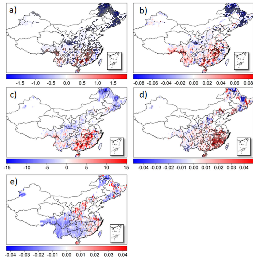
Fig. 3 Spatial patterns of trends for disturbance regimes within each 0.5° grid cell across China's forests. (a) total annual disturbed forest area ( \text{km}^2 \text{yr}^{-1} ), (b) percent of forest disturbed annually ( \% \text{yr}^{-1} ), (c) disturbance frequency (# of patches per 1000 \text{km}^2 forest), (d) mean patch size ( \text{ha yr}^{-1} ), and (e) fire severity ( \Delta\text{NDVI yr}^{-1} , delta Normalized Difference Vegetation Index). Points indicated a significant trend at 0.05 levels for disturbance regimes.
