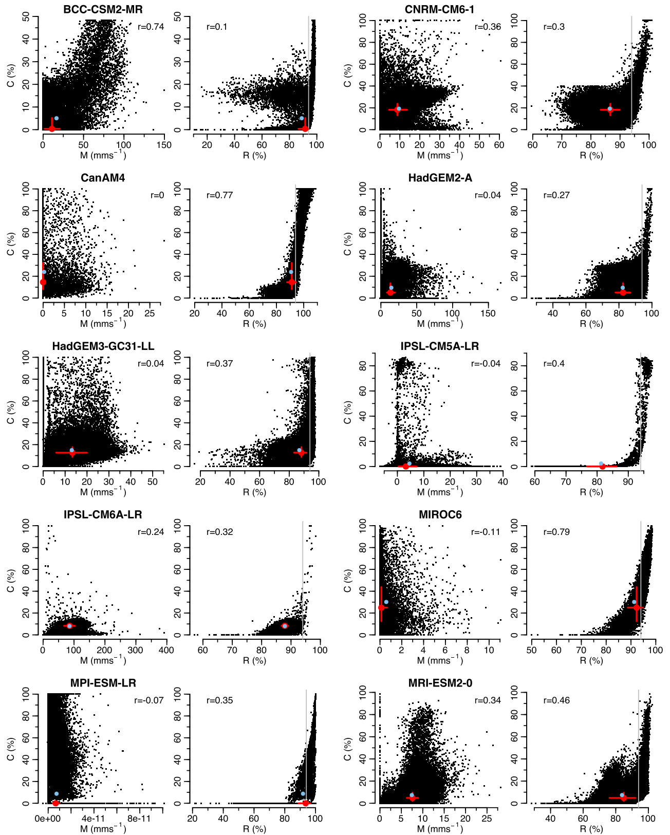
Extended Data Fig. 7 | Individual relationships of C , M and R for climate models. Relationships among individual 3-h C and M (first and third columns) and C and R (second and fourth columns) for all ten climate models. The red
