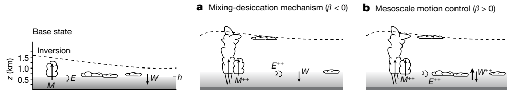
Fig. 1 | Illustration of two mechanisms for the coupling of mixing and cloudiness. a , The mixing-desiccation mechanism contends that E increases in response to an increase in M , which leads to a reduction in \mathcal{R} and cloud-base
