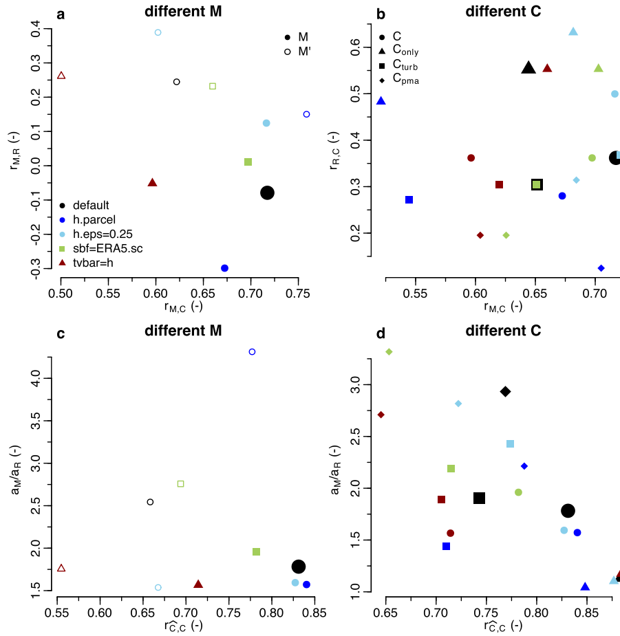
Extended Data Fig. 5 | Influence of different M and C estimates on key relationships. Correlation coefficients r of M and C ( r_{M,C} ) and M and \mathcal{R} ( r_{M,R} ) (a) and M and C ( r_{M,C} ) and \mathcal{R} and C ( r_{R,C} ) (b). c,d, Correlations of the reconstructed \hat{C} = a_0 + a_M \bar{M} + a_R \bar{R} and the observed C ( r_{\hat{C},C} ), as well as the ratio of the
