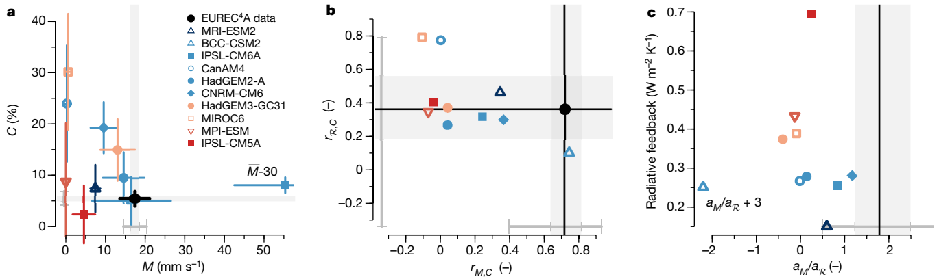
Fig. 4 | Relationships in climate models and link to trade cumulus feedback. a , Mean \pm \sigma/2 of M and C . b , Correlation coefficients r between M and C ( r_{M,C} ) and C and R ( r_{C,R} ). c , Ratio of the standardized multiple linear regression coefficients a_M/a_R and the thermodynamic component of the trade cumulus radiative feedback. The models are coloured in bins of feedback strength. Open symbols refer to models with frequent stratocumulus (defined as having
