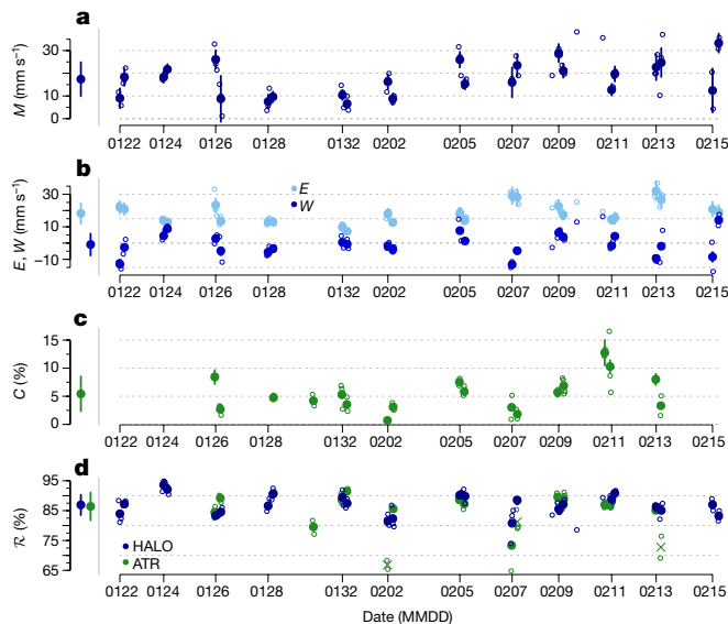
Fig. 2 | Timeseries of mixing and cloudiness during EUREC 4 A. a–d , Measurements of M ( a ), E and W ( b ) and \mathcal{R} ( d ), with filled symbols representing the 3-h scale and open symbols representing the 1-h scale. The vertical bars in a–c show the estimation uncertainty at the 3-h scale (see Methods section ‘Uncertainty estimation’). The \mathcal{R} in d is shown for both the HALO (blue) and ATR (green) aircraft, with the ‘X’ markers representing the data points that are excluded in the correlations owing to inconsistent sampling of the mesoscale cloud patterns between the two aircraft. The campaign mean \pm 1\sigma is shown on the left side of each panel.
