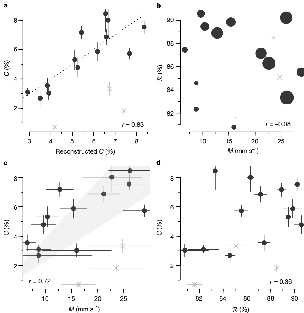
Fig. 3 | Relationships among M , R and C . a–d , The relationships between the observed C and the reconstructed \hat{C} from the regression \hat{C} = a_0 + a_M \tilde{M} + a_R \tilde{R} ( a ), M and R ( b ), M and C ( c ) and R and C ( d ) are shown at the 3-h scale. The error bars represent the estimation uncertainty for M and C and the sampling uncertainty for R (see Methods). The dotted line in a is the 1:1 line. The size of the markers in b
