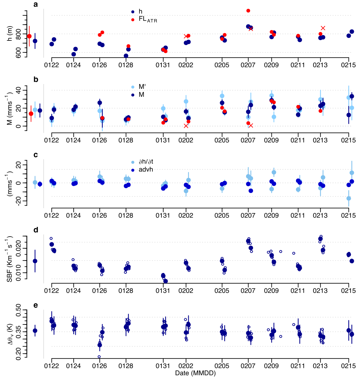
Extended Data Fig. 3 | Time series of other mass budget terms. Shown are h and the flight level of the ATR aircraft (a), the equilibrium M , the total M' and the M_{turb} from ATR turbulence measurements (b), the temporal fluctuation and advection terms (c), the surface buoyancy flux (d) and the \Delta \theta_v (e). The vertical bars show the estimation uncertainty at the 3-h scale (see Methods section
