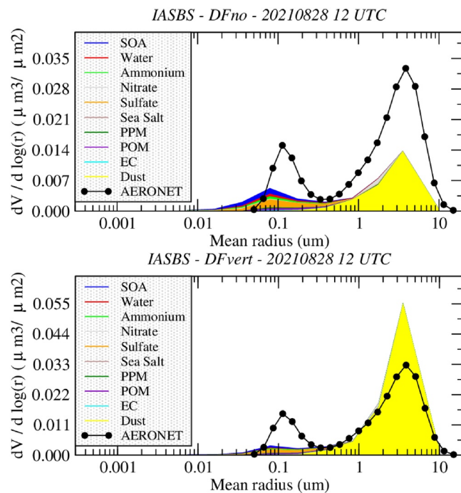
Figure 22. Aerosol size distribution, with the aerosol composition, at IASBS for the 28 August 2021 12:00 UTC and for the DFvert simulation.
