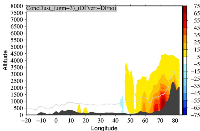
Figure 13. Vertical cross-sections of mineral dust concentrations as differences DFvert minus DFno. Values are time-averaged for latitudes between 35^\circ and 45^\circ\text{W} and for the period 15–31 August 2021. The gray line indicates the mean averaged value of the boundary layer.
