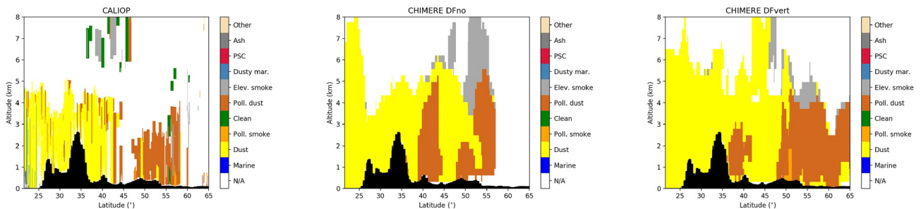
Figure 14. Comparison of vertical transects measured by the CALIOP lidar aboard CALIPSO and the two CHIMERE simulations DFno and DFvert, for the 16 August 2021, 08:40 UTC and 26 August 2021, 22:23 UTC.
