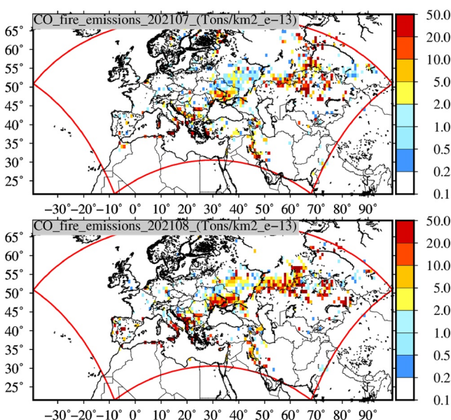
Figure 7. Cumulative fire fluxes during the months of July and August 2021 for carbon monoxide, CO (molecules cm^{-2} s^{-1} \times 10^{-15} ).
