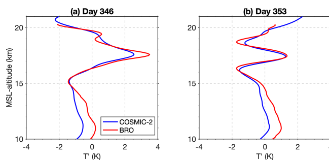
Figure 12. Profiles of Kelvin wave temperature perturbations from COSMIC-2 and BRO from Fig. 11c and d, on (a) day 346 when the 6 km vertical wavelength dominates and (b) day 353 when the 3 km wavelength dominates.
