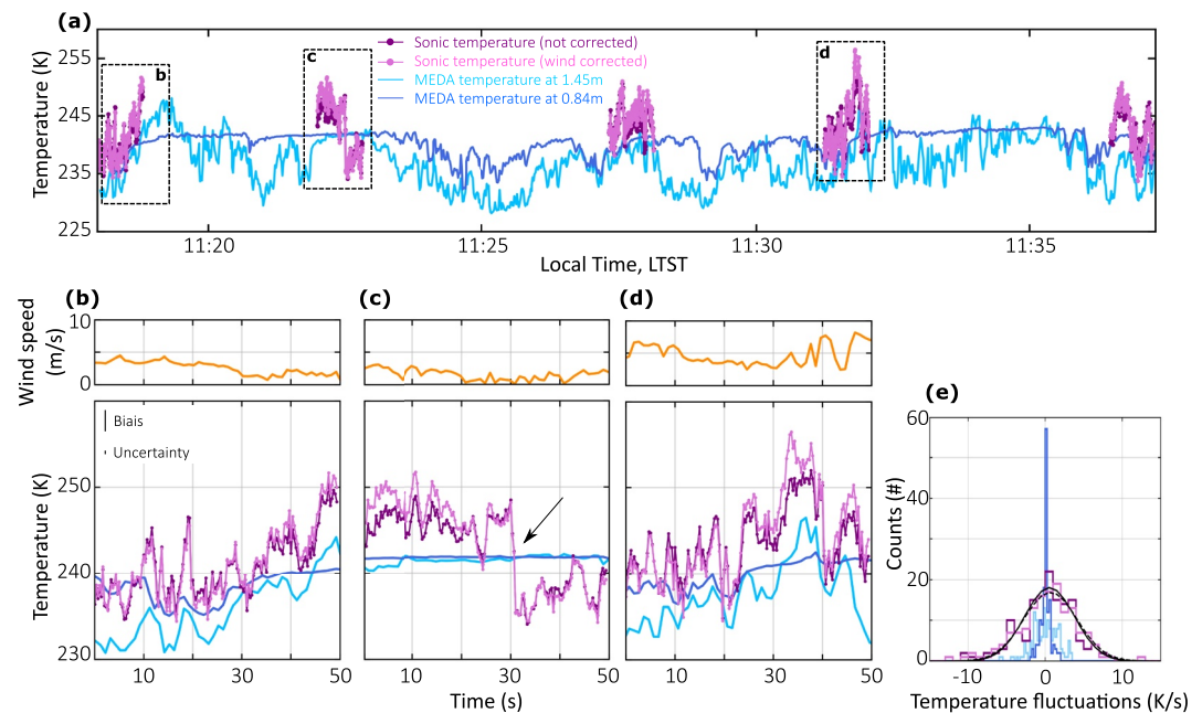
Figure 3. (a) Evolution of the sonic temperature for target Vilette (Sol 189, 5 points of 150 laser shots each), compared with Mars Environmental Dynamics Analyzer (MEDA) temperatures at 1.45 and 0.84 m. (b–d) Close-up views of the three 50 s long bursts indicated in panel (a) and compared with MEDA temperature and wind measurements. The top left vertical bars indicate the error budget: the bias corresponds to the error on the distance, the uncertainty corresponds to the uncertainty on the propagation time (see Texts S4 and S5 in Supporting Information S1). The arrow in panel (c) indicates the temperature drop discussed in the main text. (e) Histogram of the time derivative temperature over the data displayed in panel (d). Microphone data (both wind corrected in pink and not in purple) are fitted with a Gaussian distribution, in solid and dotted lines, respectively.
