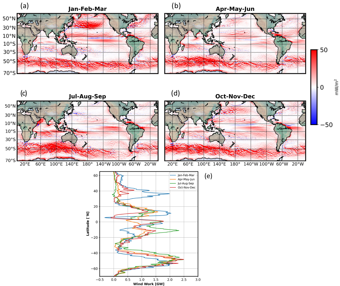
Figure 4. (a–d) Time-mean component of the wind work, \overline{\tau \cdot \mathbf{u}_0} , in different seasons. (e) Wind work multiplied by the area of the numerical grid cell ( \text{m}^2 ) and zonally integrated during the four seasons.
