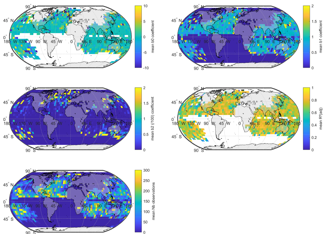
Figure A3. Map of latitude variation mean coefficients fitted on a 5 \times 5 grid grouped per month.
