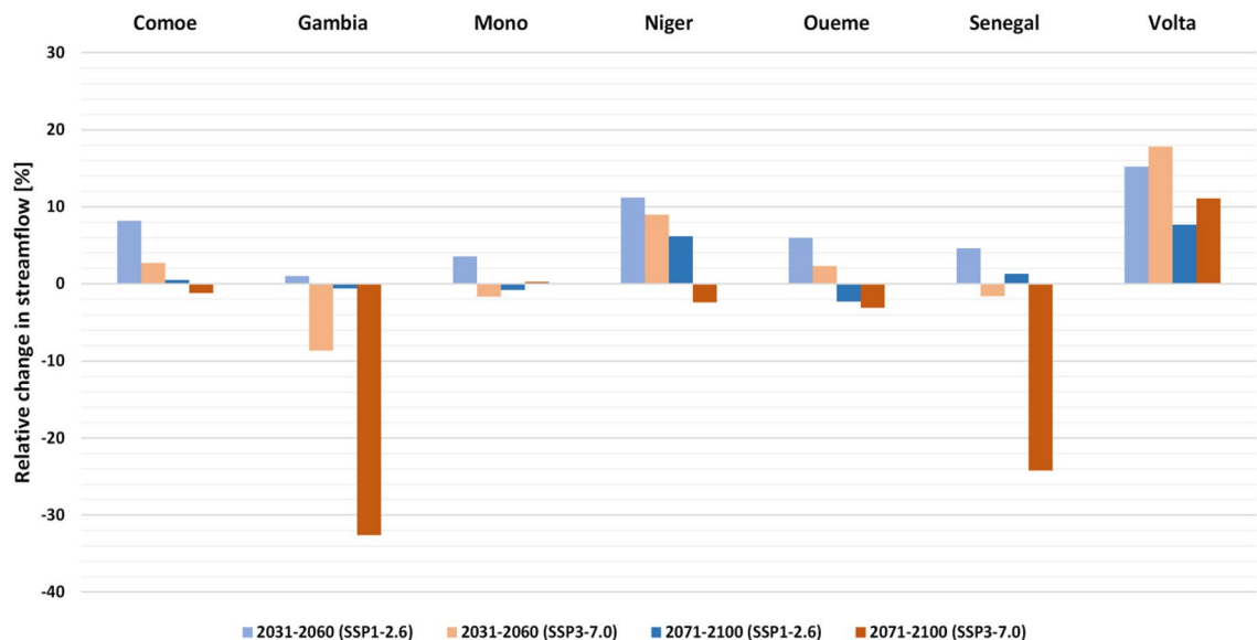
Figure 2. Changes in streamflow (%) relative to the 1981–2010 baseline for seven major river basins in West Africa.
