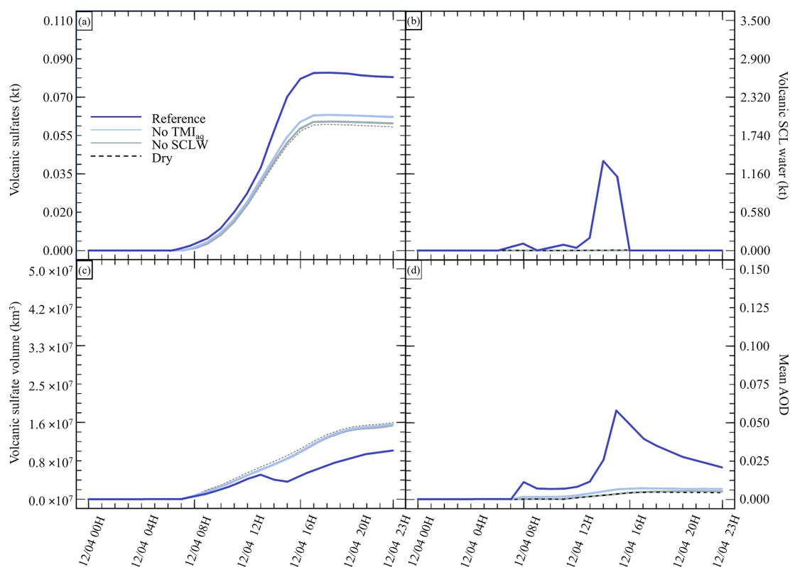
Figure 2. Sensitivity tests on chemistry parameters for (a) sulfate aerosols ( \text{SO}_4^{2-} , kt), (b) supercooled liquid water (kt), (c) the minimum volume ( \text{km}^3 ) \subset 25 % of \text{SO}_4^{2-} mass and (d) the AOD for plume \subset 25 % of \text{SO}_4^{2-} mass. The Reference simulation is the closest to a realistic case. All time series represent differences relative to the Background simulation (the simulation without volcanic emissions).
