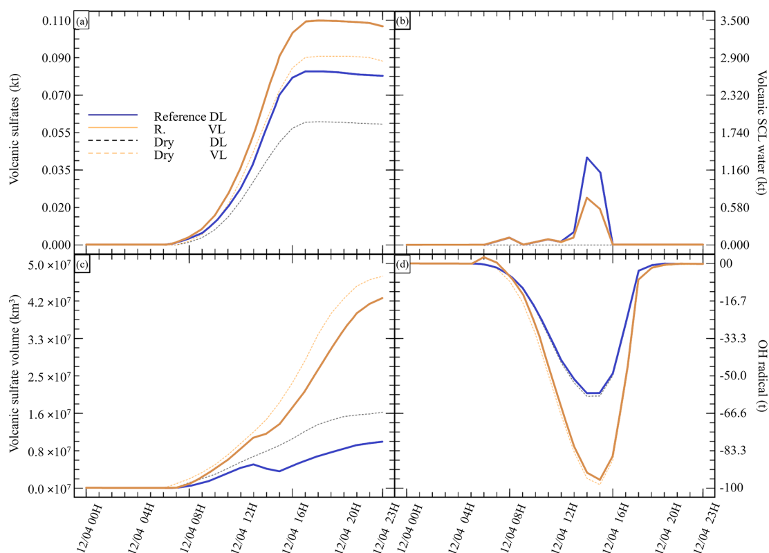
Figure 6. Sensitivity tests on injection height for (a) sulfate aerosols ( \text{SO}_{4(p)}^{2-} , kt), (b) supercooled liquid water (kt), (c) the minimum volume ( \text{km}^3 ) \subset 25 % of \text{SO}_{4(p)}^{2-} mass and (d) the OH radical (t). The Reference simulation is the closest to a realistic case. All time series represent differences relative to the Background simulation (the simulation without volcanic emissions).
