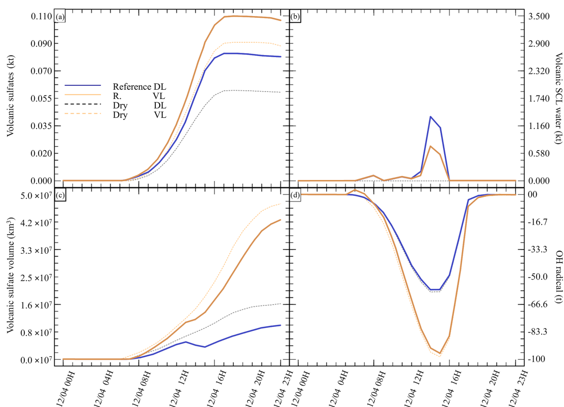
Figure 6. Sensitivity tests on injection height for (a) sulfate aerosols (SO 4(p) 2- , kt), (b) supercooled liquid water (kt), (c) the minimum volume (km 3 ) < 25 % of SO 4(p) 2- mass and (d) the OH radical (t). The Reference simulation is the closest to a realistic case. All time series represent differences relative to the Background simulation (the simulation without volcanic emissions).
