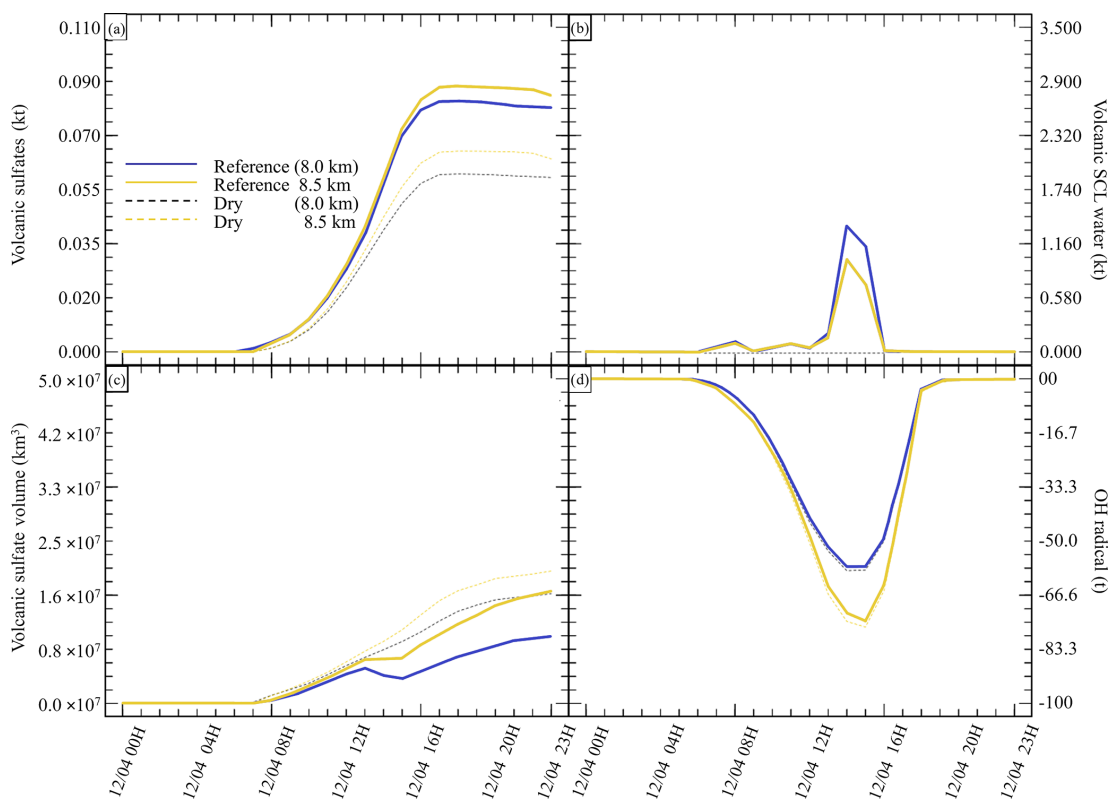
Figure 5. Sensitivity tests on injection height for (a) sulfate aerosols (SO 4 2- , kt), (b) supercooled liquid water (kt), (c) the minimum volume (km 3 ) < 25% of SO 4 2- mass and (d) OH radical (t). The Reference simulation is the closest to a realistic case. All time series represent differences relative to the Background simulation (the simulation without volcanic emissions).
