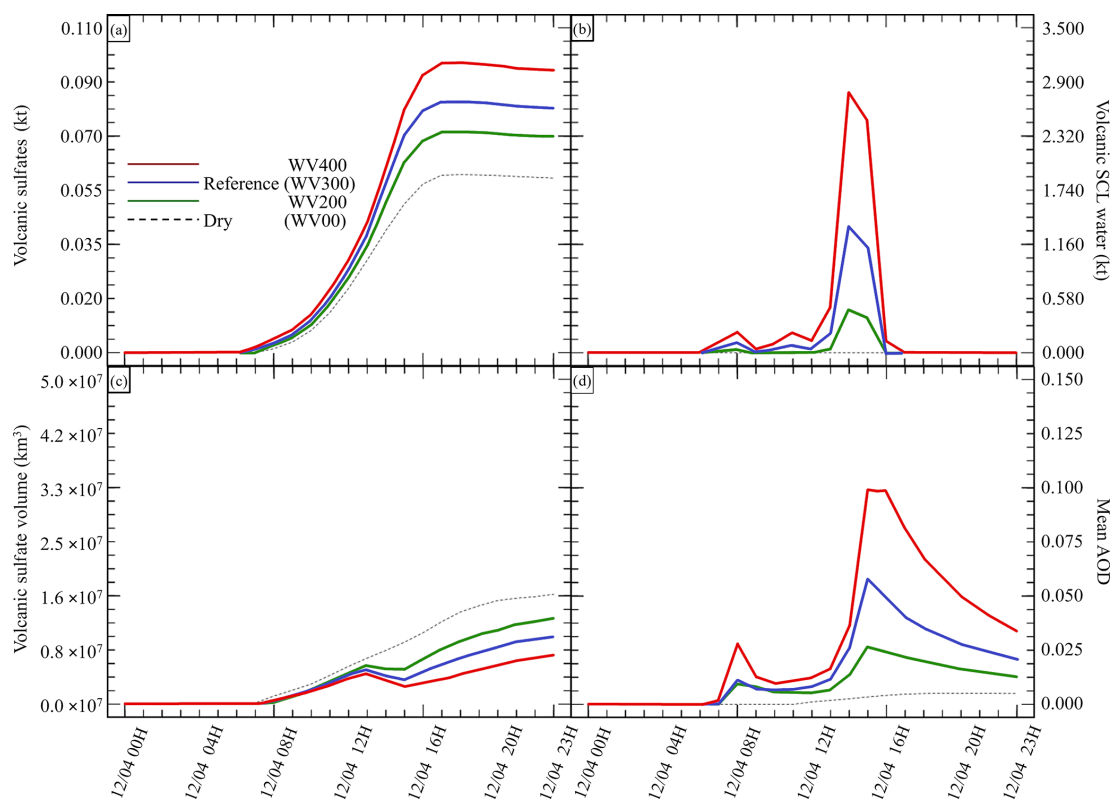
Figure 3. Sensitivity tests on volcanic water emissions for (a) sulfate aerosols (SO 4(p) 2- , kt), (b) supercooled liquid water (kt), (c) the minimum volume (km 3 ) < 25 % of SO 4(p) 2- mass and (d) the AOD for plume < 25 % of SO 4(p) 2- mass. The Reference simulation is the closest to a realistic case. All time series represent differences relative to the Background simulation (the simulation without volcanic emissions).
