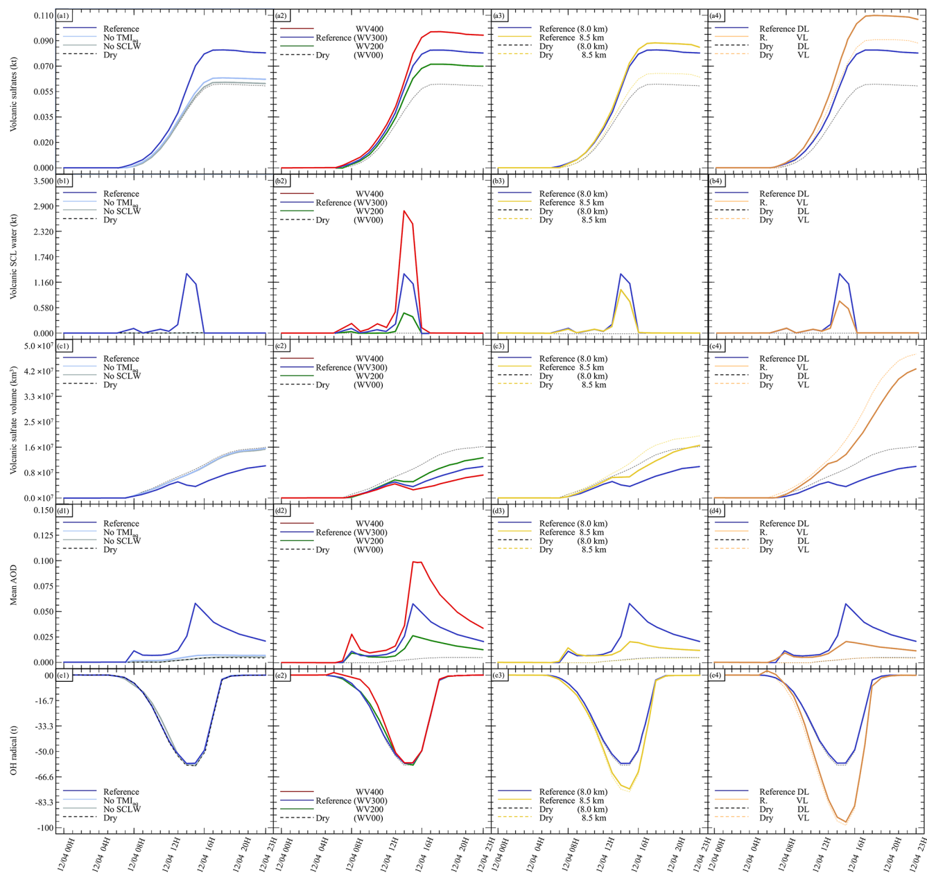
Figure A5. Results from the various simulations performed with respect to (a) \text{SO}_{4(p)}^{2-} (kt), (b) supercooled liquid water (kt), (c) the minimum volume ( \text{km}^3 ) \subset 25 % of \text{SO}_{4(p)}^{2-} mass, (d) the AOD for plume \subset 25 % of \text{SO}_{4(p)}^{2-} mass and (e) the OH radical (t). The Reference simulation is the closest to a realistic case.
