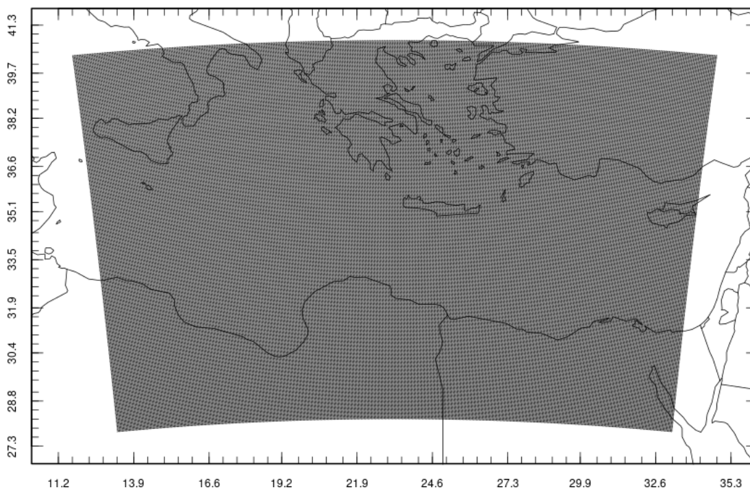
Figure A2. The CHIMERE simulation domain contains 874 × 624 cells at a 2.25 km resolution.
