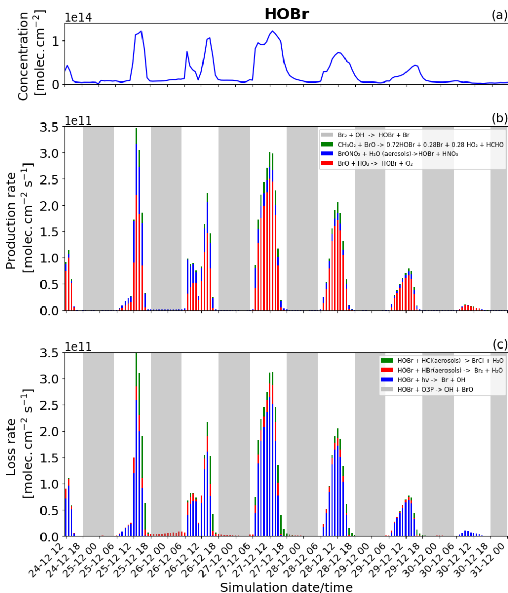
Figure 10. Time evolution of (a) HOBr column concentration in molecules per square centimetre (molec. cm -2 ), (b) production rates, and (c) loss rates for HOBr with both the production and loss shown in molecules per square centimetre per second (molec. cm -2 s -1 ) from 24 December at 12:00 UTC to 31 December 2018 at 00:00 UTC in the near-volcano plume.
