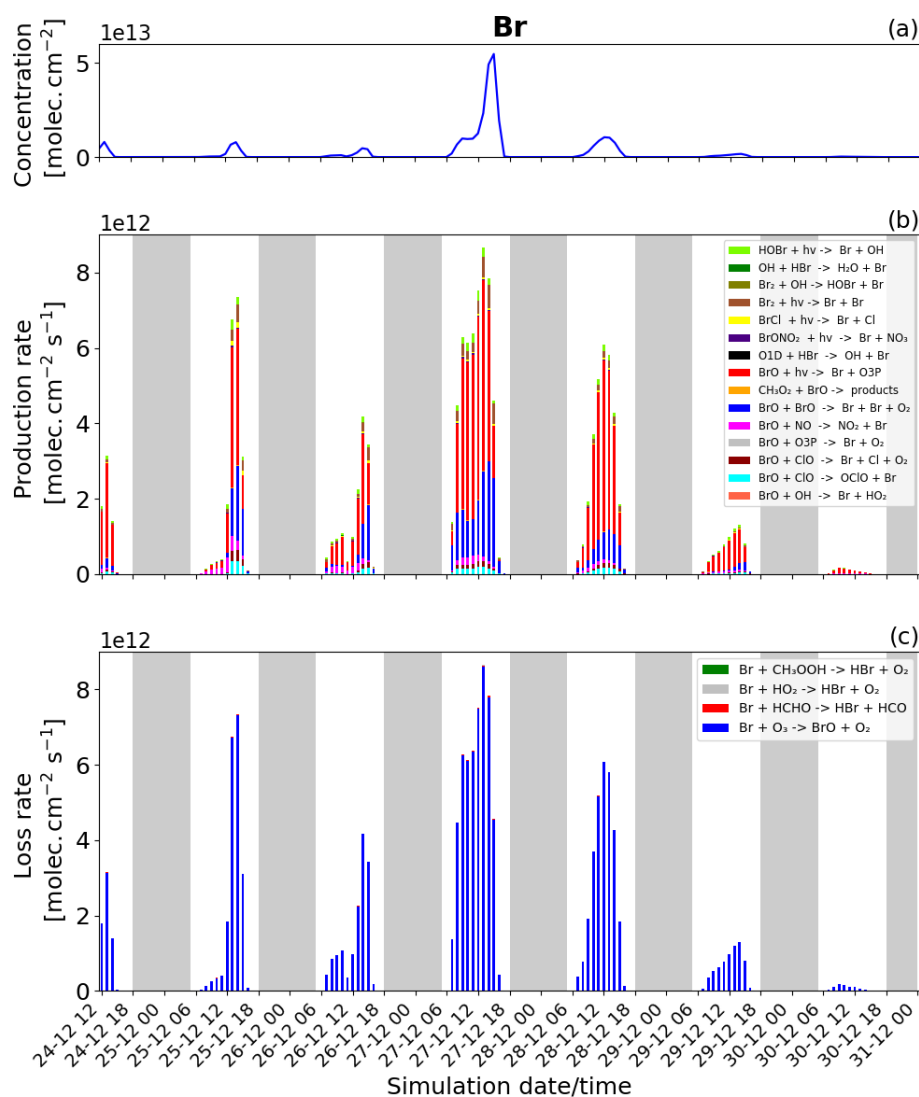
Figure 7. Time evolution of (a) Br column concentration in molecules per square centimetre (molec. cm -2 ), (b) production rates, and (c) loss rates for Br with both the production and loss shown in molecules per square centimetre per second (molec. cm -2 s -1 ) from 24 December at 12:00 UTC to 31 December 2018 at 00:00 UTC in the near-volcano plume.
