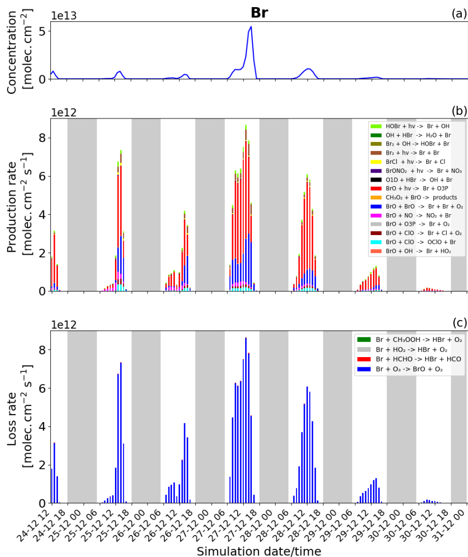
Figure 7. Time evolution of (a) Br column concentration in molecules per square centimetre (molec. cm -2 ), (b) production rates, and (c) loss rates for Br with both the production and loss shown in molecules per square centimetre per second (molec. cm -2 s -1 ) from 24 December at 12:00 UTC to 31 December 2018 at 00:00 UTC in the near-volcano plume.
