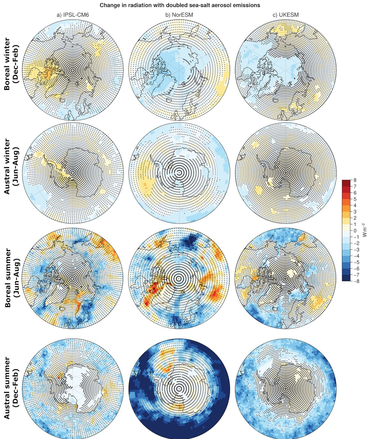
Figure 10. Change in top-of-atmosphere net downward radiative flux ( rtmt ) in a scenario with doubled sea salt aerosol emissions under pre-industrial atmospheric composition (30 years under 1850 conditions). Stippling shows the grid points for which the difference between piClim-2xss and piClim-control is not significant at the 90% level according to a Wilcoxon test.
