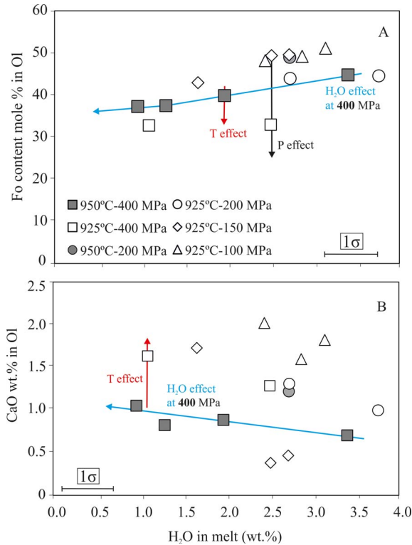
Figure 5. Composition of experimental olivine. (A) Fo content, (B) CaO (wt%) in Ol versus H 2 O melt . Vertical errors are equal to size symbols.
