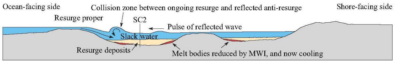
Fig. 6. Schematic process reconstruction of Stage 5 of the resurge at the Rochechouart crater (Fig. 4). As currently the size and morphology of the fresh crater are not known, the cross-section is only meant to be seen as conceptual in order to explain the various interpreted mechanisms of the resurge process, e.g. collision of flow, MWI, pulse of reflected wave. The conceptual cross-section chosen here is that of a complex crater, as the consensus of current published estimates is that of a crater with a diameter much wider than the transition from simple to complex morphology. However, in a much larger option, the central uplift indicated here could be replaced by a peak ring. The location of the drill hole SC2 is indicated, as well as the likely nearshore position of the crater.
