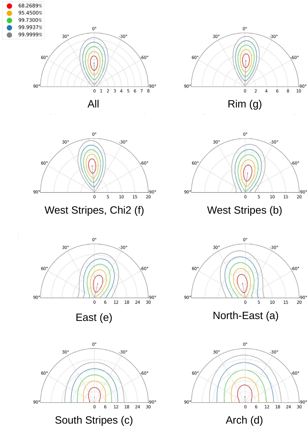
Figure 4. Polar plots for the Tycho regions of interest considered in this work. Each diagram depicts the measured degree of polarization and direction with respect to a circular symmetry and the geometrical center of the remnant, as confidence contours for the regions listed in Table 1. The confidence levels given are color coded in the legend. The radial coordinate indicates the degree of polarization in percent. Values more consistent with a direction of polarization of 0^\circ correspond to an overall tangentially oriented polarization averaged over the region.
