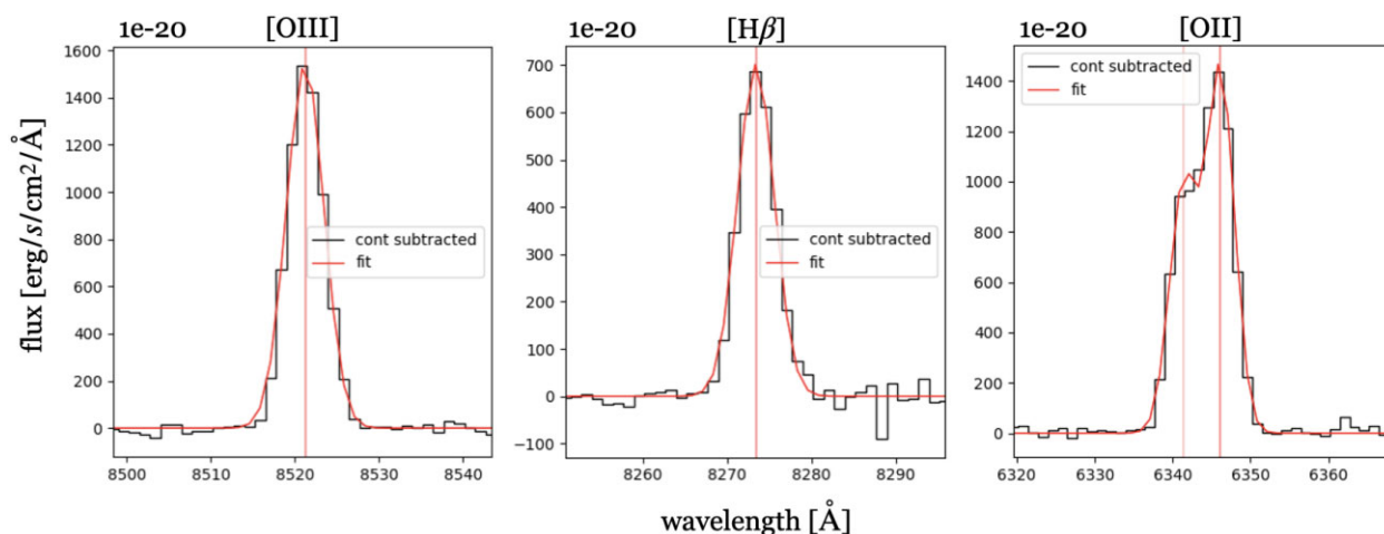
Figure A1. One high SNR example of MUSE spectra of the lines used in this work, namely [O III], H \beta , and [O II] (galaxy 211130). The black line shows the continuum-subtracted spectrum, the red line shows the fit and the vertical red line shows the position of the peak, in all panels.
