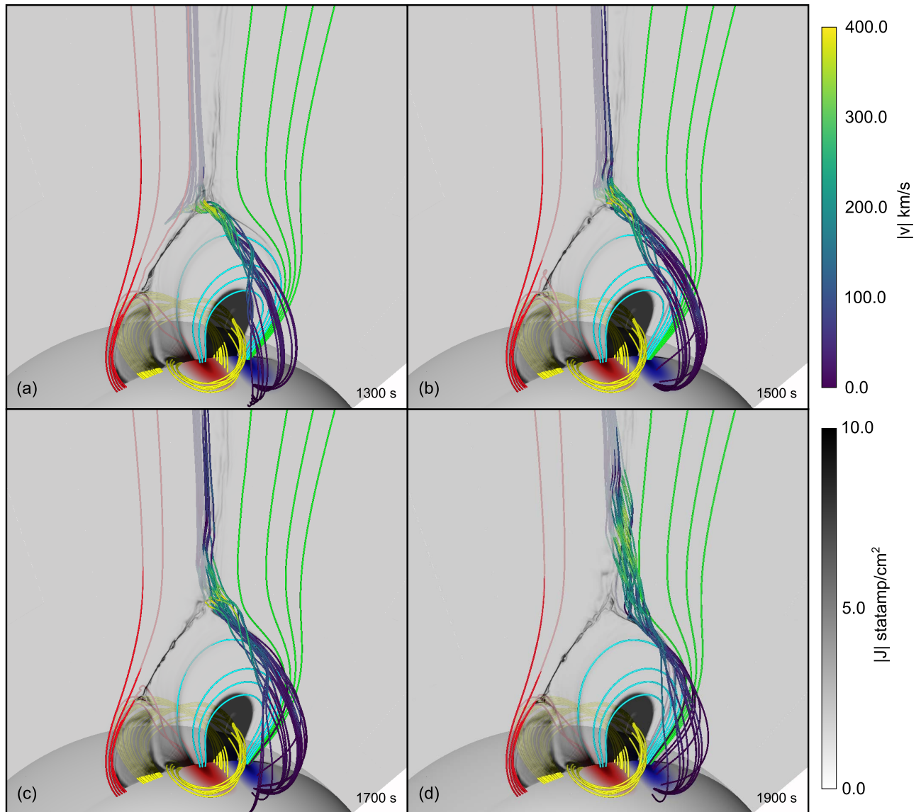
Figure 3. Field lines within the plasmoid flux rope highlighted with the red arrow in Figure 2(c) as it is ejected from the current layer. The field lines are colored (blue/green) according to the local plasma velocity magnitude. Note that the field lines are chosen to show the twist evolution within the flux rope and differ between times. The gray shading shows |J| as in Figure 2(a).
