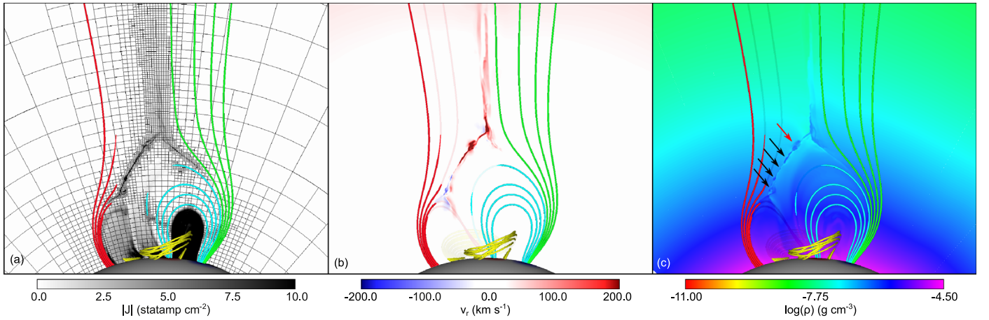
Figure 2. (a) Current density |J| overlaid with the outline of the grid blocks at t = 1100 s, (b) v_r , and (c) \log(\rho) highlighting the increased density within the plasmoid flux ropes. Field lines in the filament channel (yellow) and regions of closed inflow (cyan), open inflow (red), and open outflow (green) to/from the current layer are shown for reference. Each panel contains field lines traced in 3D together with the distribution of the corresponding quantity in a vertical plane ( \phi = 1.3^\circ ) that approximately aligns with the reconnection inflows/outflows. An animation of panel (a) is available showing the plasmoid evolution. The duration is 6 s and runs from t = 0 to 3600 s.
