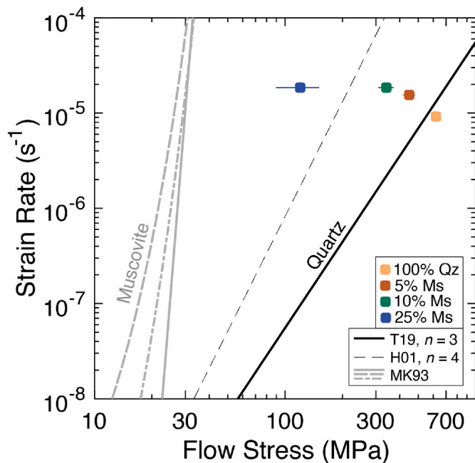
Fig. 17. Plot of log strain rate versus log stress comparing the high strain mechanical data with quartz and muscovite flow laws. The three grey curves are muscovite flow laws developed based on the mechanical data from Mares and Kronenberg (1993) - MK93. The dashed curve (the weakest flow law) is the exponential relationship developed by Mares and Kronenberg (1993). The dash-dot curve is an exponential flow law developed in this study incorporating a stress squared term and the solid line is a power law flow law developed in this study (for flow law parameters, see text). The solid black curve represents the quartz flow law defined by Tokle et al. (2019) - T19 - where A = 8.3e-13 \text{ MPa}^{-n} \text{ s}^{-1} and the black dashed curve represents the quartz flow law defined by Hirth et al. (2001) - H01. We use a water fugacity of 4840 MPa for the quartz flow laws. The shear stresses and shear strain rates for the four high strain samples were converted to equivalent stresses and strain rates. Error bars of \pm 30 \text{ MPa} are plotted following Holyoke and Kronenberg (2010).
