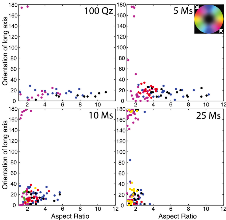
Fig. 14. Plots of aspect ratio versus orientation of the long particle axis for the high strain samples. Data are color-coded to represent the particle (e.g., grains) c-axis orientation. The color lookup table is represented in the top right of figure. 0 and 180 represent the orientation of the shear plane. SURFOR analyses were performed on relict quartz grains from the CIP maps in Fig. 13. The white arrows around the color look up table define the axial shortening direction. Long axis angle orientations follow the same convention used in Fig. 10. (For interpretation of the references to color in this figure legend, the reader is referred to the Web version of this article.)
