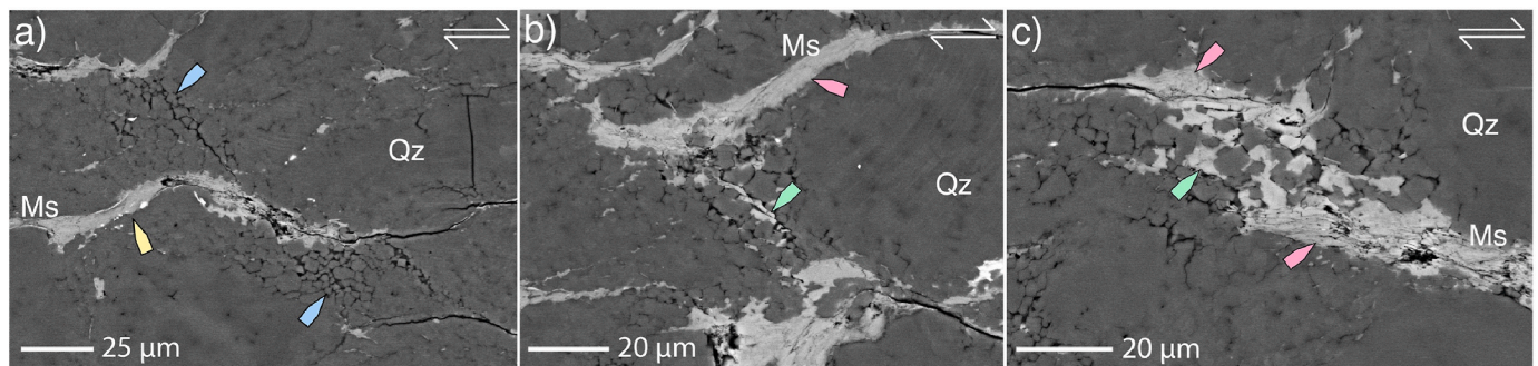
Fig. 9. Backscatter Electron images of C'-bands in the 10% muscovite sample that originate and terminate at the tip of muscovite grains. a) C'-bands are largely made of equant quartz grains and surrounded by void space highlighted by blue arrows. b) An example of neocrystallized muscovite (green arrows) mixing with recrystallized quartz grains and c) shows an example where there is significant mixing between neocrystallized muscovite (green arrow) and recrystallized quartz. b, c) Red arrows highlight relict/original muscovite grains. The yellow arrow in a) highlights potential reaction products from muscovite compositional change. The shear plane is parallel with the horizontal plane of each micrograph with a dextral sense of shear. Muscovite (Ms) grains are lighter grey and quartz (Qz) darker grey. Portions of muscovite grains are plucked during sample preparation. (For interpretation of the references to color in this figure legend, the reader is referred to the Web version of this article.)
