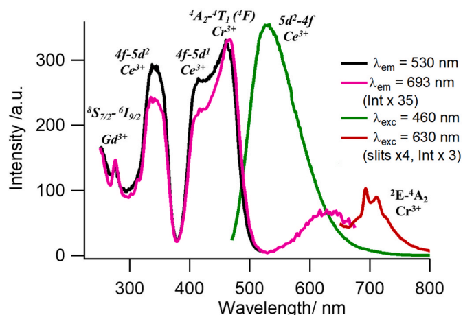
Fig. 3. Excitation and fluorescence spectra of (\text{Gd}_{0.61}\text{Y}_{0.39})_{3.02(4)}\text{Ce}_{0.008(1)}(\text{Al}_{2.30(3)}\text{Ga}_{2.67(3)}\text{Cr}_x)\text{O}_{12} .
