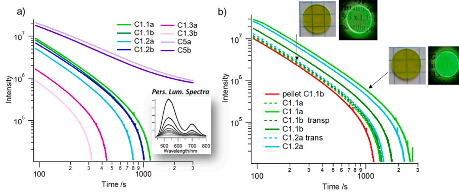
Fig. 6. Integrated Persistent luminescence intensity of (\text{Gd}_x\text{Y}_x)_3\text{Ce}_x(\text{Al}_2\text{Ga}_3\text{Cr}_x)\text{O}_{12} after excitation at 295 K with a 455 LED (1150 mW) during 10 min for the crystals a) with different composition (Inset: Persistent luminescence spectra) and b) with different volume and transparency.
