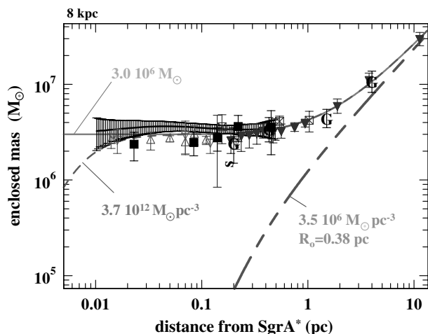
Figure 17. Mass distribution in the central 10 pc of the Galaxy obtained from stellar and gas dynamics (for R_{\odot} = 8.0 kpc). The different data points (all with \pm 1\sigma uncertainties) are as follows. Bold ‘G’ denotes mass estimates from the ionized and neutral gas dynamics (Serabyn & Lacy 1985; Güsten et al. 1987; Lacy et al. 1991; Herbst et al. 1993; Roberts & Goss 1993). Rectangles with crosses and down-pointing triangles denote the isotropic mass modelling of Genzel et al. (1996, 1997), including Jeans modelling of stellar radial velocities (early- and late-type stars, filled down-pointing triangles) and Bahcall–Tremaine estimators of the NTT proper motions until 1996 (open down-pointing triangles). Open rectangles (with crosses) are Bahcall–Tremaine estimators of the line-of-sight-velocity data only. Open up-pointing triangles are the Bahcall–Tremaine estimators of the 1995–1996 proper motion data of Ghez et al. (1998). The new anisotropy-independent mass estimates from the present work are given as filled black rectangles (Leonard–Merritt estimators of the proper motions in (Tables 1 and 2) and as large black crosses connected by a continuous curve (Jeans model, Table 5). For comparison several model curves are shown. The long–long–short dashed curve (green in the colour version of the figure reproduced in Synergy ) represents the mass model for the (visible) stellar cluster [ M/L(2\ \mu\text{m}) = 2 , r_{\text{core}} = 0.38 pc, \rho(r=0) = 3.5 \times 10^6\ \text{M}_{\odot}\ \text{pc}^{-3} ]. The continuous curve (light blue in the colour version of the figure reproduced in Synergy ) is the sum of this stellar cluster, plus a point mass of 3.0 \times 10^6\ \text{M}_{\odot} . The short dashed curve (red in the colour version of the figure reproduced in Synergy ) is the sum of the visible stellar cluster, plus an \alpha = 5 Plummer model, \rho(r) = \rho(0)[1 + (r/r_0)^2]^{-\alpha/2} , of a dark cluster of central density 3.7 \times 10^{12}\ \text{M}_{\odot}\ \text{pc}^{-3} and r_0 = 0.0058 pc.
