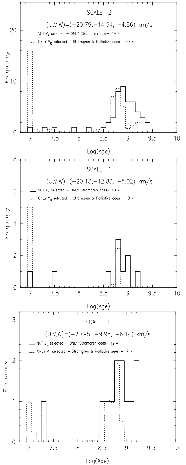
Fig. 20. IC 2391 SCl. Age distributions for the IC 2391 SCl (stream 2-14 in Table 3) at scale 2 (top), for sub-stream 1-20 (in Table 4) at scale 1 (middle) and for sub-stream 1-25 (in Table 4) at scale 1 (bottom)
