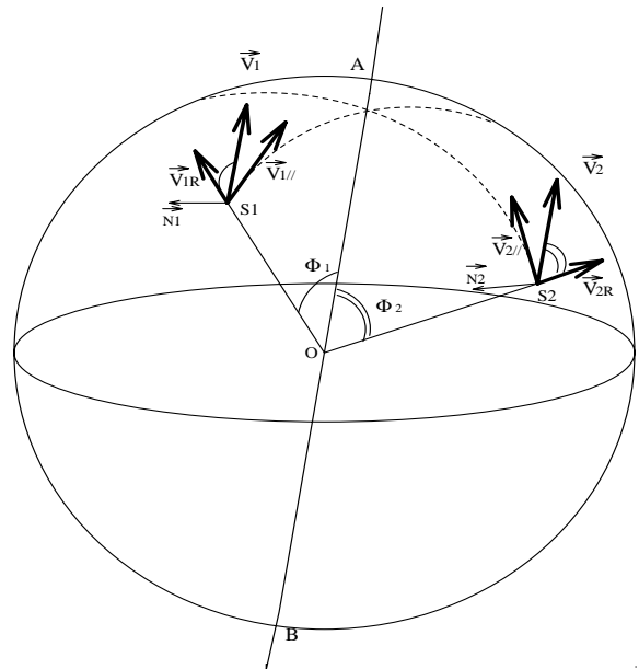
Fig. 11. Implementation of the convergent point method. \vec{V}_{1\parallel} , \vec{V}_{2\parallel} are the tangential velocities measured by Hipparcos for two stars. \vec{V}_{1R} , \vec{V}_{2R} are deduced radial velocities assuming that stars S_1 and S_2 belong to the same stream
