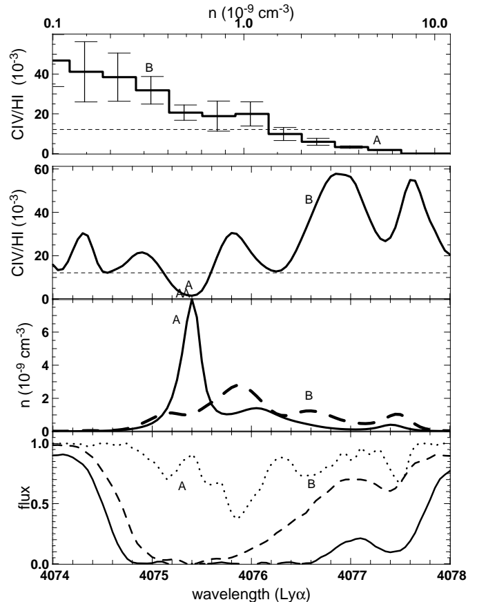
Fig. 17. Determination of the C IV/H I ratio along the absorption profile of the strong complex at \lambda 4076 Å (see also Fig. 16). Bottom panel: Lyman- \alpha (solid line), Lyman- \beta (dashed line) and C IV (scaled by a factor 4, dotted line) absorption profiles. Second panel: recovered H I (solid line) and C IV (scaled by the average C IV/H I ratio, dashed line) density (see text for details about the reconstruction). Third panel: C IV/H I ratio; the horizontal line indicates the ratio of the C IV and H I integrated densities. Top panel: the C IV/H I ratio is plotted versus the H I density. The markers A and B correspond to positions discussed in the text.
