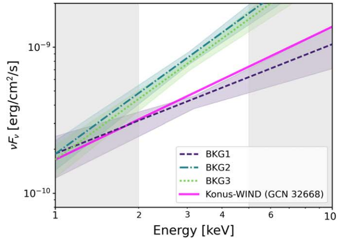
Figure 5. Left: best-fit average distance of the dust clouds. The orange bands are centered on the average of the best-fit values weighted by their uncertainties, and have a width representative of the mean relative statistical error for the two dust clouds responsible for r_1 and r_2 emissions. Right: derived intrinsic GRB prompt spectrum. The light-gray regions cover the energy ranges excluded in the fitting procedure. In both plots, the colors violet, teal, and green correspond to the different assumed backgrounds BKG1, BKG2, and BKG3, respectively.
