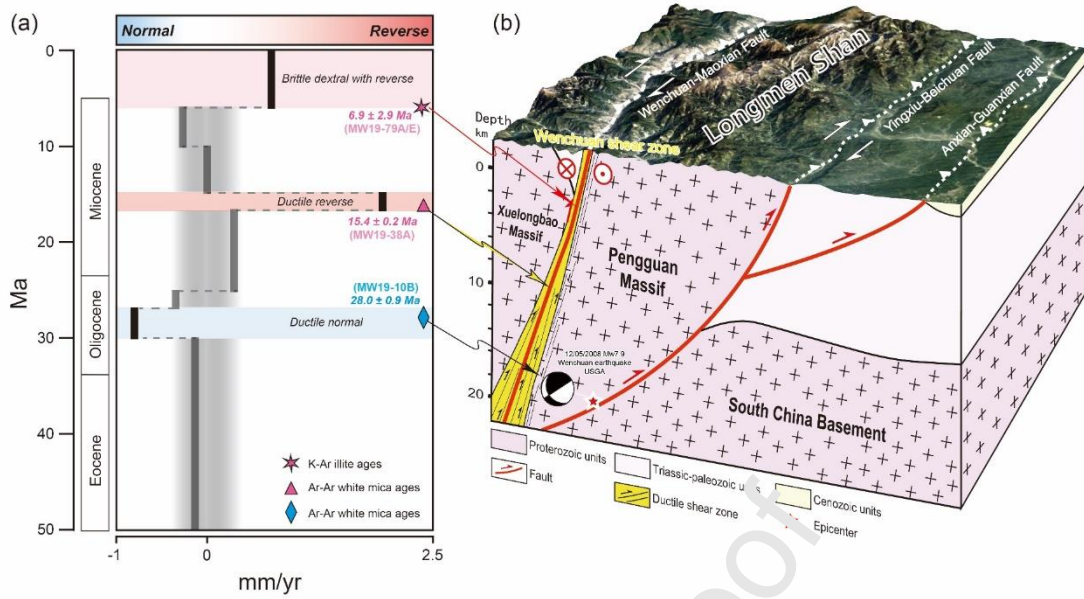
Fig. 10 Kinematics of the Wenchuan-Maowen fault. (a) vertical differential exhumation across the fault according to thermochronological data of the Pengguan and Xuelongbao ranges (Furlong et al., 2021; Wang et al., 2012). Negative values correspond to normal motion on the NW dipping fault, and positive to reverse motion. (b) structural block diagram of Longmen Shan in shallow crust.
