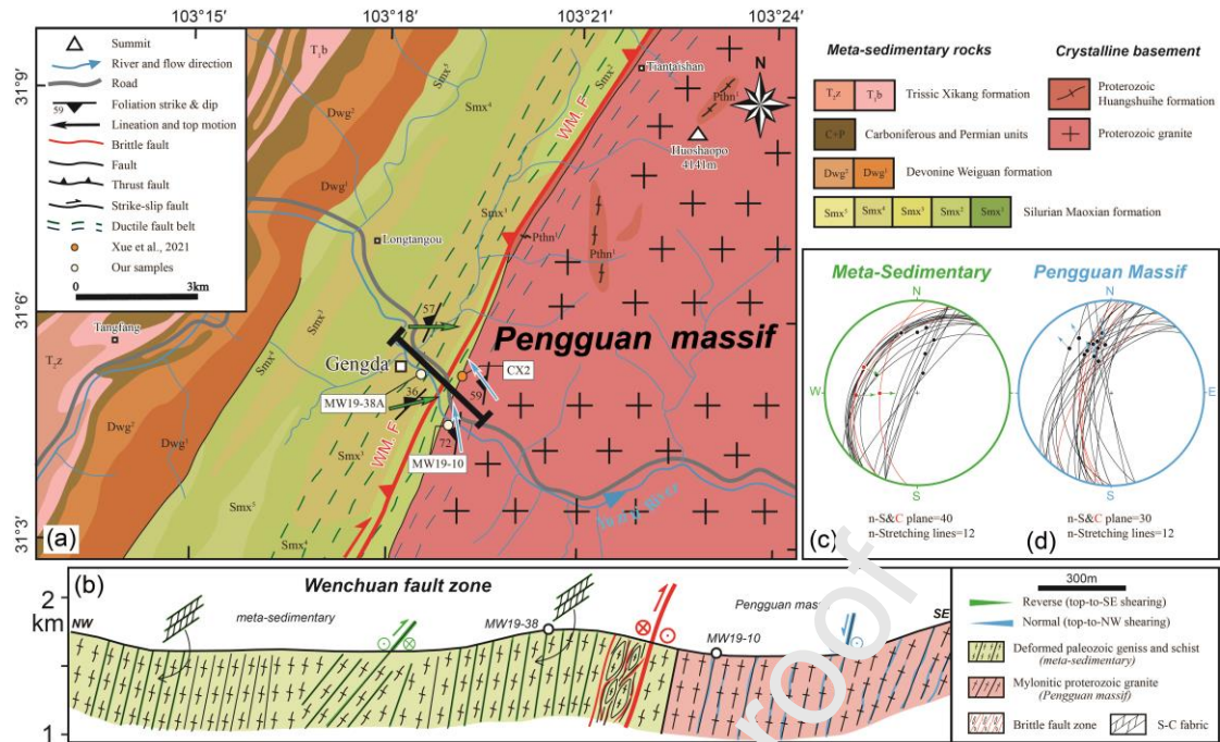
Fig. 4 Ductile deformation in the WM fault zone. a) Geological map of the Gengda area of the WM fault zone. See location on fig. 1(b). b) Geological cross section through the WM fault and shear zones. c, d) Stereonet diagram of foliations and shear planes on the western side of the fault (c) and on the eastern side (d).
