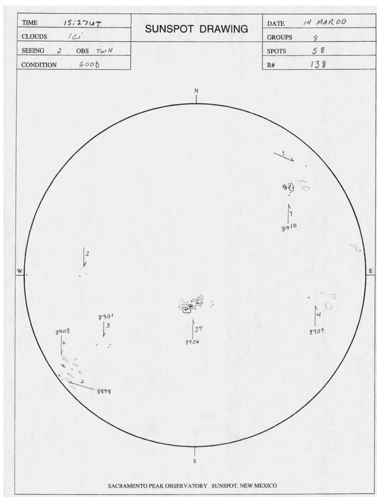
Figure 1b Sunspot drawing by Tim Henry from the US National Solar Observatory at Sacramento Peak on 14 March 2000, about 7 hours after the Locarno observation in Figure 1a. Eight groups and 58 sunspots were observed to yield S_N (Sacramento Peak) = 138. Fainter contours outline photospheric faculae, visible near the solar limb. ( ngdc.noaa.gov/stp/space-weather/solar-data/solar-imagery/photosphere/sunspot-drawings/sac-peak/ )
