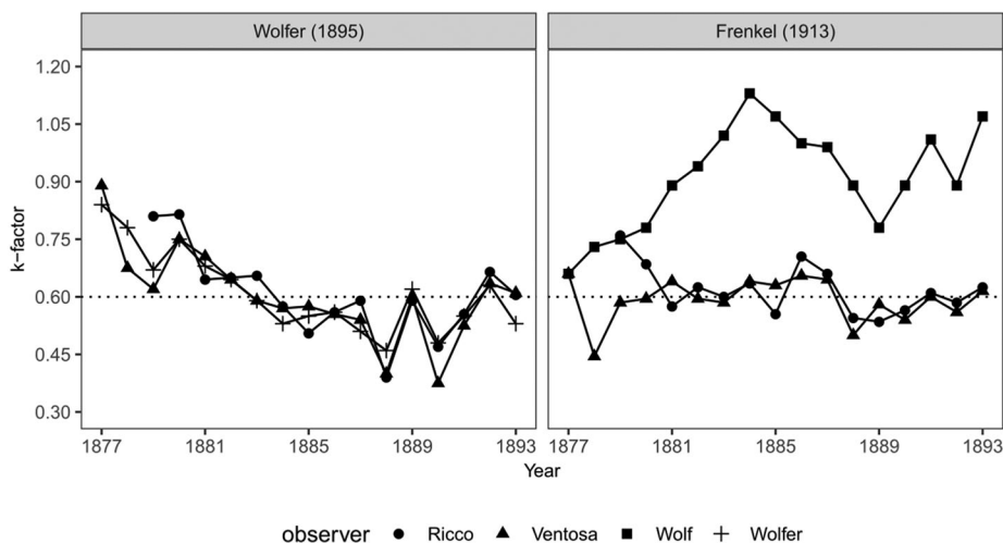
Figure 4 Left panel: yearly k -factors of Ricco, Ventosa, and Wolfer relative to Wolf as given by Wolfer (1895), showing a clear drift before 1884. Right panel: yearly k -factors of Ricco, Ventosa, and Wolf as given by Frenkel (1913) using Wolfer as reference. The k factors are stable over the whole time interval, indicating that all observers are stable. By contrast, the yearly k -factor of Rudolf Wolf, with the small portable refractor relative to the numbers from Wolfer using the 83-mm standard Zürich refractor (squares), shows the same trend between 1877 and 1884, but also a modulation that follows the solar cycle (minima in 1879 and 1890, maxima in 1884 and 1894) (from Friedli, 2020).
