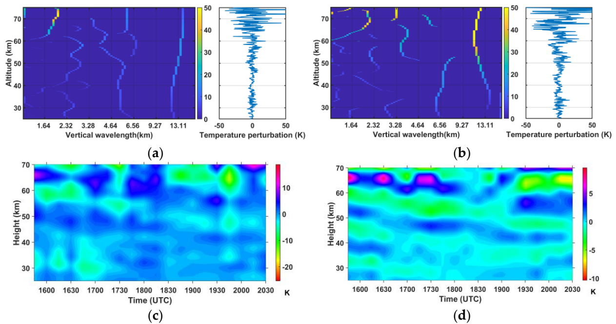
Figure 10. Spectral lines for the CWT maxima with values >5% of the maximum CWT-coefficient absolute value derived from 15 min lidar temperature perturbation profiles on (a) 9 October at 1835 UTC (2235 LST) and (b) 10 October at 1645 UTC (2045 LST); Height-time variation of perturbations on 9 October with vertical wavelengths (c) >5 km and of (d) 9.6–19.2 km.
