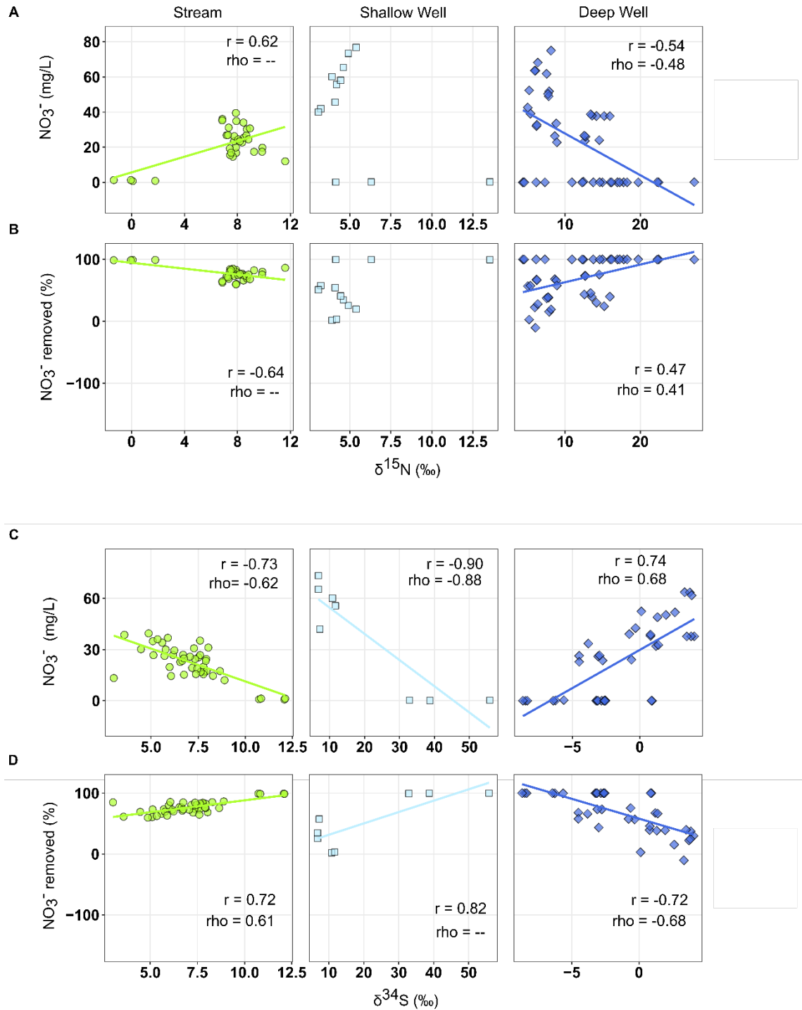
Figure 5. Relationships of \delta^{15}\text{N} and \delta^{34}\text{S} with \text{NO}_3^- concentration and removal. Linear fit lines are shown for convenience to indicate a significant relationship—either Pearson ( r ) or Spearman ( \rho )—at \alpha = 0.05 .
