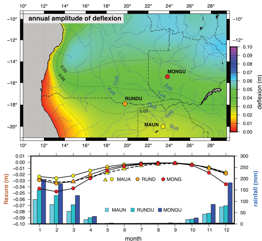
FIGURE 4 Flexure induced by water mass present in the study area. The hydrological budget integrates the rainfall and the water previously stored pondered by a coefficient (see text for explanation). The upper map displays the annual range of vertical displacement. The dotted deflection curves are spaced every 1 cm. The lower plot illustrates the monthly variations of vertical displacement of the three GPS sites, and the vertical bars illustrate the monthly rainfall at each site. The dashed line with yellow triangles shows the monthly flexure at Maun considering 6% of water storage in the Okavango Delta.
